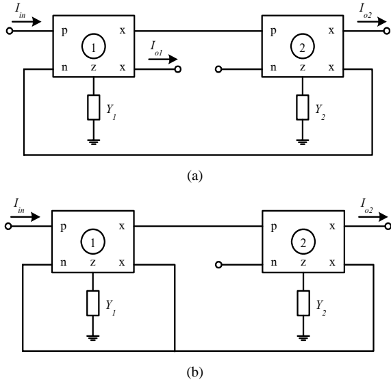
Fig. 3 : Proposed topology 1 (a) Case 1 (b) Case 2
