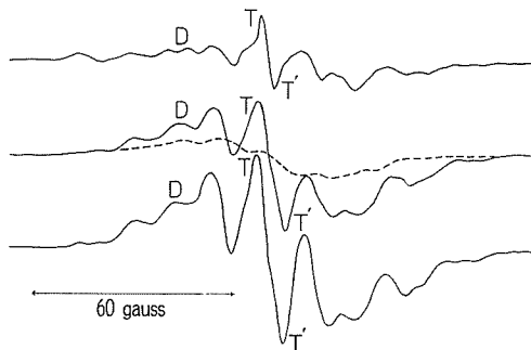
Fig. 3. ESR spectra of irradiated dichloromethane.
