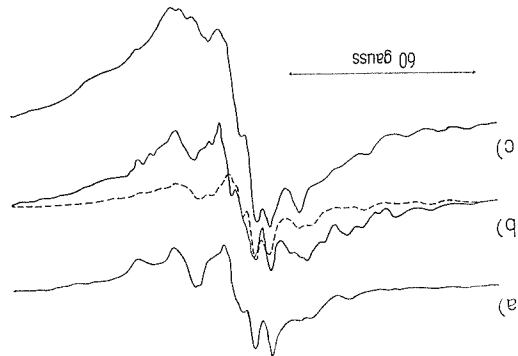
Fig. 2. ESR spectra of irradiated trichloromethane.
