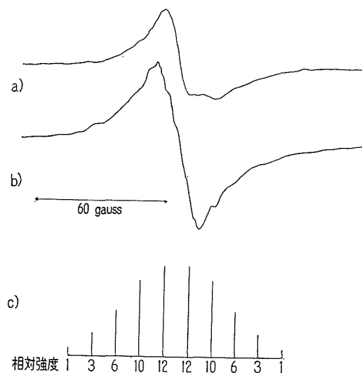
Fig. 1. ESR spectra of irradiated carbon tetrachloride.
