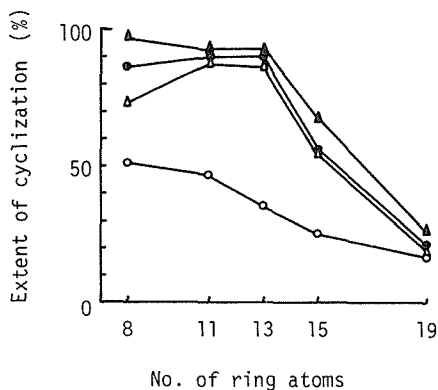
Figure 9. Polymerization of oligomethylene acrylates: (○) with AIBN at 60°C; (△) in the presence of AlEt 2 Cl at 40°C, Al/M 1.0; (●) in the presence of AlEt 1.5 Cl 1.5 at 40°C, Al/M 1.0; (▲) in the presence of AlEtCl 2 at 40°C, Al/M 1.0.
