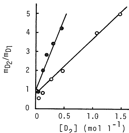
Figure 8. Plots of m_{D_2}/m_{D_1} against the D_2 concentration: (○) for the system of o -allylphenyl acrylate - p -chlorostyrene; (●) for the system of 2-( o -allylphenoxy)ethyl acrylate - p -chlorostyrene.
