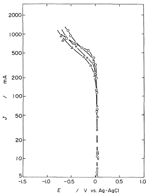
Fig. 4 Polarization curves for various electrodes with pre-electrolysis in 100 ppm \text{Cu}^{2+} solution. \omega = 700 rpm, Q = 3.4 \text{ l} \cdot \text{min}^{-1} . Pre-electrolysis potential (V vs. Ag-AgCl): \triangle = -0.14 , \times = -0.20 , \circ = -0.25 , and \square = -0.40 .
