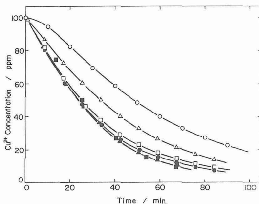
Fig. 6 Concentration variation with time in 30 l of 100 ppm \text{Cu}^{2+} solution with various pre-electrolyzed electrodes. J=0.5 A, \omega=700 r.p.m., Q=3.4 l \text{min}^{-1} . The quantity of electricity for the pre-electrolysis (coulomb): \circ=0 , \triangle=1000 , \square=2000 , \bullet=3000 , \blacktriangle=6000 , and \blacksquare=10000 .
