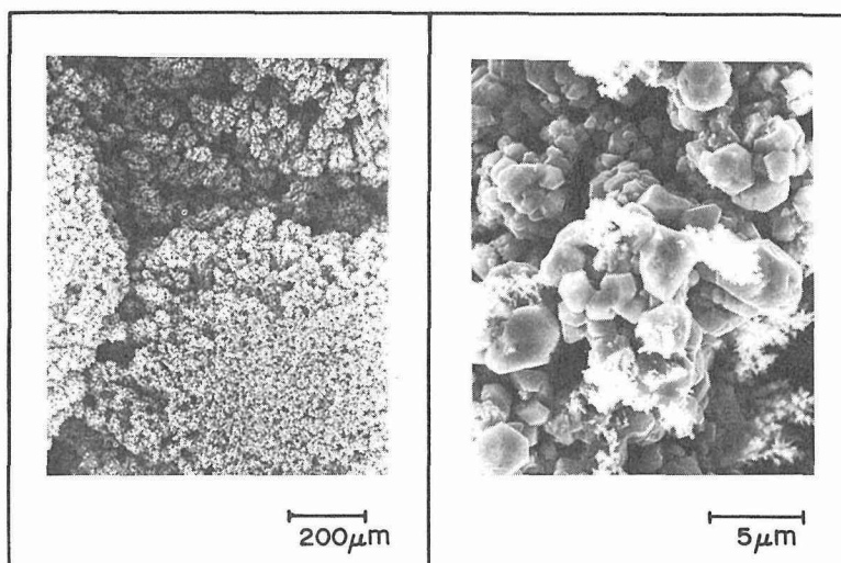
Photo. 1 SEM photographs of surface of deposited copper at -0.14 V and 25000 coulombs.
