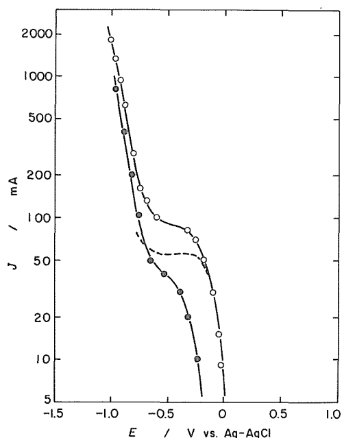
Fig. 2 Polarization curves on smooth copper electrode. \omega = 700 rpm, Q = 3.4 l \text{min}^{-1} \circ = 100 ppm \text{Cu}^{2+} with 5 \times 10^{-2} M \text{H}_2\text{SO}_4 , and \bullet = 5 \times 10^{-2} M \text{H}_2\text{SO}_4 only.
