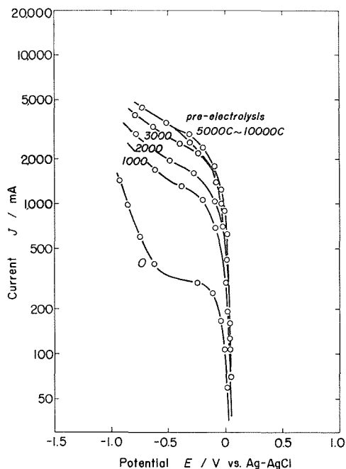
Fig. 5 Polarization curves at various quantities of electricity for pre-electrolysis at about -0.25 V in 500 ppm \text{Cu}^{2+} solution. \omega = 700 rpm, Q = 3.4 \text{ l} \cdot \text{min}^{-1} .
