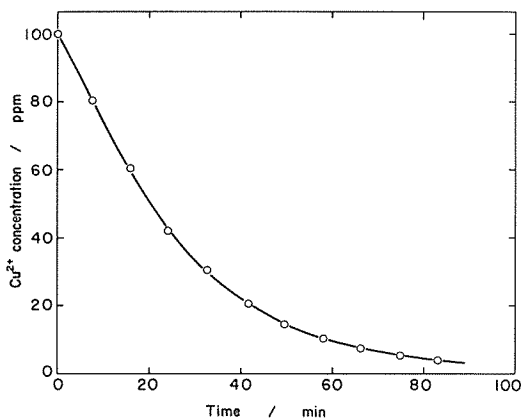
Fig. 8 Concentration variation with time in 30 l of 100 ppm \text{Cu}^{2+} solution with pre-electrolysis as schem 2 in Table 1. J=0.5 \text{ A} , \omega=700 \text{ rpm} , Q=3.4 \text{ l} \cdot \text{min}^{-1} .
