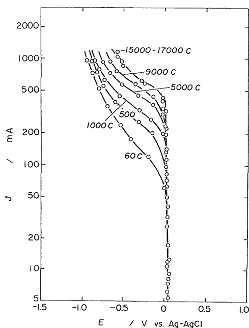
Fig. 3 Polarization curves at various quantities of electricity for pre-electrolysis at -0.25 V in 100 ppm \text{Cu}^{2+} solutions. \omega = 700 rpm, Q = 3.4 l \text{min}^{-1} .
