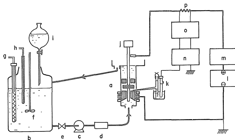
Fig. 1 Apparatus and measurement system for polarization curves. a = test cell, b = reservoir tank, c = pump, d = flow meter, e = valve, f = impeller, g = heater, h = thermocouple, i = 1 M CuSO 4 solution, j = motor, k = Ag-AgCl electrode, l = power supply, m = coulometer, n = high impedance voltmeter, o = recorder, p = standard resistance.
