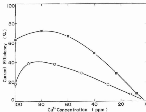
Fig. 7 Current efficiency variations with \text{Cu}^{2+} concentration on different pre-electrolyzed electrodes. J=0.5 A, \omega=700 rpm, Q=3.4 l \text{min}^{-1} . The quantity of electricity for pre-electrolysis(coulomb): \circ=0 , and \bullet=10000 .
