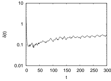
Figure 8. Time evolution of the analyticity strip \delta(t) up to t = 300 for \alpha = 0.4 , \nu = 1.0 \times 10^{-3} in a semi-log plot.
