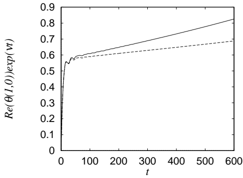
Figure 26. Time evolution of a Fourier coefficient compensated by \exp(\nu t) with \nu = 1.0 \times 10^{-3} , for supercritical \alpha = 0.4 (solid) and subcritical \alpha = 0.7 (dashed).
