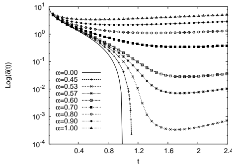
Figure 1. Time evolution of the analyticity strip \delta(t) for the Burgers equation for various values of \alpha .
