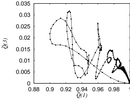
Figure 23. Phase portrait in normalised spectrum \tilde{Q}(1) - \tilde{Q}(3) for \alpha = 0.4 , \nu = 1.0 \times 10^{-3} .
