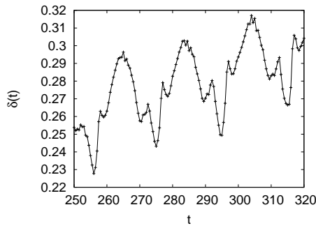
Figure 10. Time evolution of \delta(t) for \alpha = 0.4 , \nu = 1.0 \times 10^{-3} from t = 250 to 320 when the oscillatory damping is taking place.
