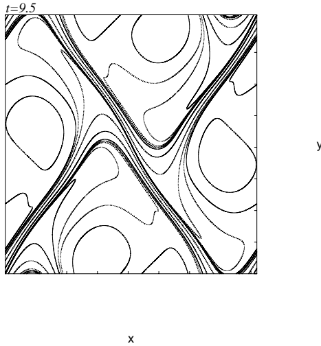
Figure 3. Contour plots of active scalar for the inviscid case at t = 9.5 in [-\pi, \pi]^2 . Equally-spaced 10 thresholds are used between the maximum and minimum.
