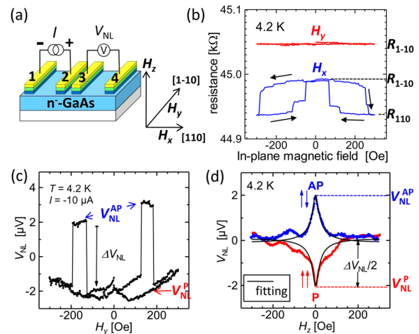
FIG. 1. (Color online) (a) Schematic device structure of a four-terminal nonlocal device and circuit configuration for non-local spin-valve and Hanle measurements. (b) Magnetoresistance curves measured at 4.2 K for a \text{Co}_{50}\text{Fe}_{50}/\text{n-GaAs} single junction under injector contact-2 through the three-terminal geometry. The bias voltage was -0.15 \text{ V} and an in-plane magnetic field along the [110]_{\text{CoFe}} direction ( H_x ) or along the [1-10]_{\text{CoFe}} direction ( H_y ) was applied. The curve for H_y has an offset of 60 \Omega for clarity. (c) Non-local voltage vs. in-plane magnetic field ( H_y ) (spin-valve signal) for a \text{Co}_{50}\text{Fe}_{50}/\text{n-GaAs} junction measured at 4.2 K. (d) Non-local voltage vs. out-of-plane magnetic field ( H_z ) (Hanle signal) for a \text{Co}_{50}\text{Fe}_{50}/\text{n-GaAs} junction measured at 4.2 K for both P (lower curve) and AP (upper curve) configurations. The solid lines are the result of the fitting from Eq. (1). In (c) and (d), the background signal was subtracted.
