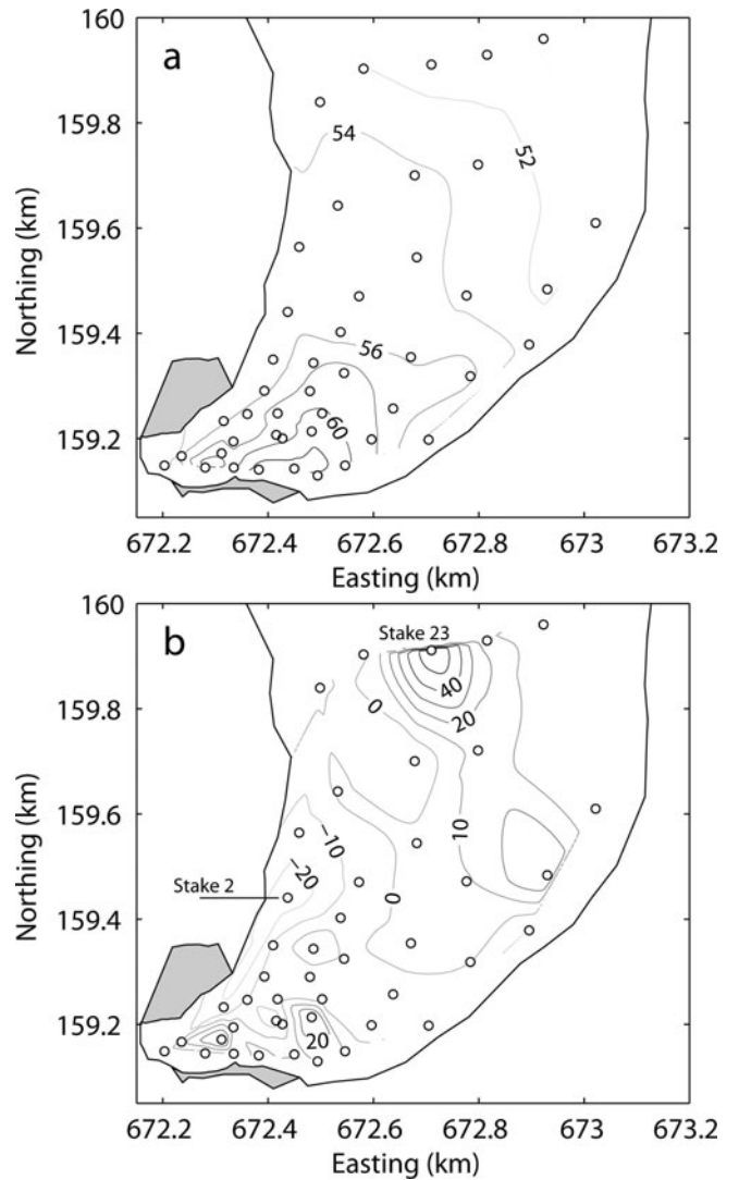
Fig. 5. (a) Melt rates ( \text{mm w.e. d}^{-1} ) computed for the period 6 July to 6 September 2009; and (b) relative deviations from the observed values, (M_{\text{comp}}/M_{\text{meas}} - 1) \times 100\% . The locations of ablation stakes are indicated by circles.
