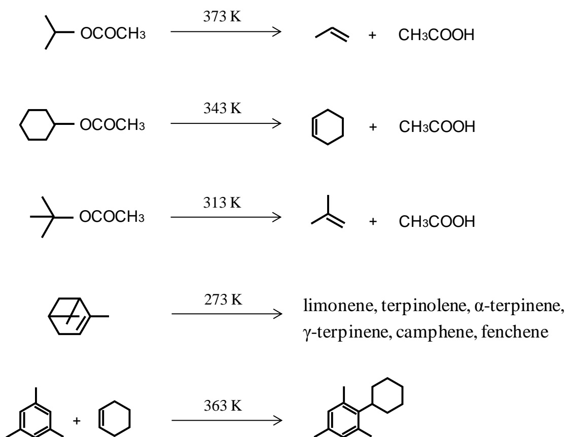
Figure S1. Catalytic reactions in a liquid-solid reaction system conducted in the present study.
