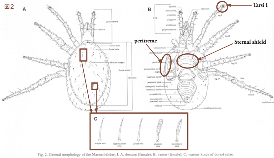
Fig. 2. General morphology of the Macrocheleidae. I. A, dorsum (female); B, venter (female); C, various kinds of dorsal setae.
