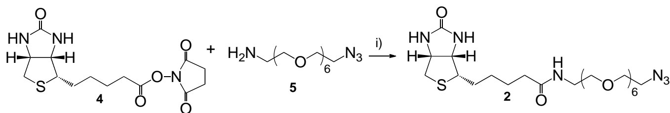
Scheme 2. Synthesis of biotin-PEG-azide derivative ( 2 ) from biotin N -hydroxysuccinimide ester ( 4 ) and H_2N -PEG-azide ( 5 ). i) TEA, DMF, rt, 12 h, 83 %.
