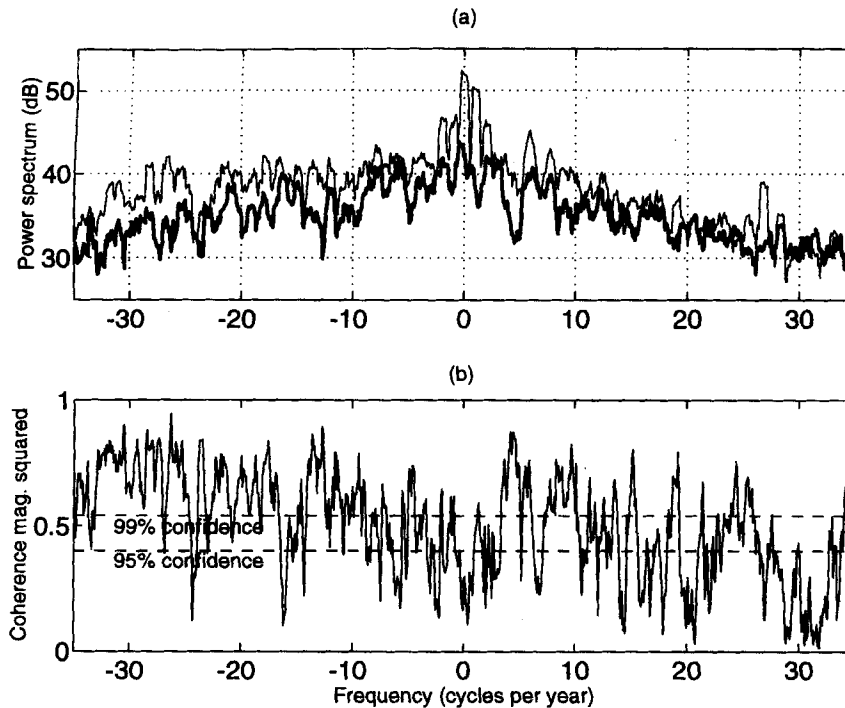
Figure 5. (a) The thin curve is the (multitapered) power spectrum of the observed polar motion excitation function (mean value removed). The thick curve is that of the non-AAM excitation function after all coherent signals and the optimal AAM are removed. (b) The coherence magnitude-squared spectrum between the observed and AAM-induced excitation functions, after all coherent signals are removed. The two horizontal lines indicate the confidence level of 99 per cent (0.54) and 95 per cent (0.40).
