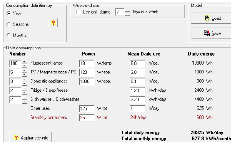
Figure 4: Daily consumption of electricity during a year, PVSYS
