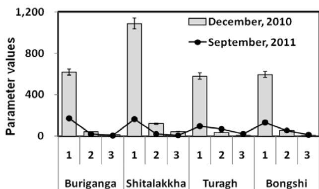
Fig. 2 Variation of general water quality in the rivers of Dhaka, Bangladesh 1= Conductivity (µS/cm); 2=COD (mg/L); 3=DOC (mg/L)
