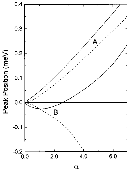
FIG. 2. Peak positions of split levels vs the ac field strength. Solid lines A and B are the energy shifts (from E_2 ) of peaks labeled by A and B on the dotted line in Fig. 1, respectively. Dashed lines show peak positions of the dashed line in Fig. 1.
