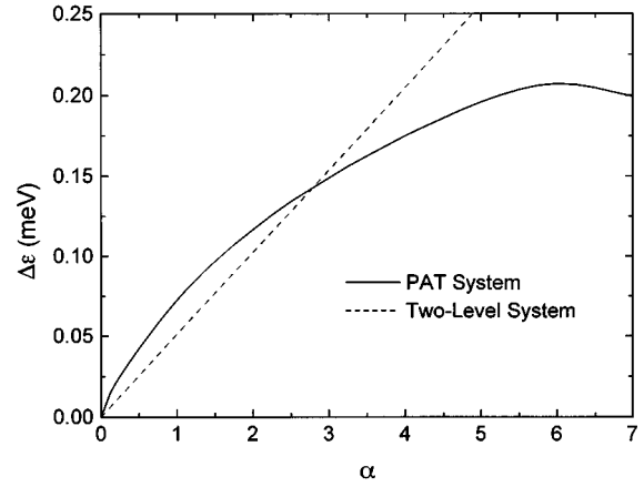
FIG. 3. Energy separation \Delta\varepsilon of split levels as a function of the ac field strength. Solid line indicates \Delta\varepsilon between resonant peaks labeled by A and B in Fig. 1. Dashed line is calculated in terms of Eq. (4.3) with d = 7 nm.
