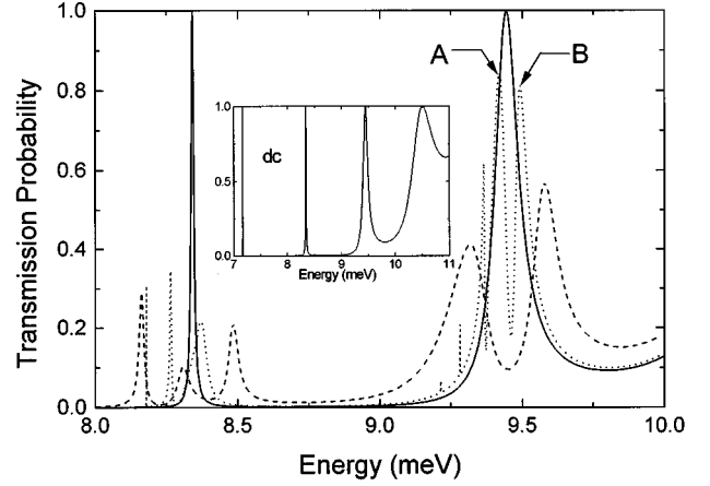
FIG. 1. Transmission probabilities for double-barrier systems ( V_0 = 10 meV, x_0 = 150 nm, and \xi = 50 nm) with and without an ac field as a function of the energy of the incident electron. Solid lines in this figure and its inset indicate the transmission probability for the static system. Dotted line shows the result for the harmonically driven system ( \hbar\omega = 1.10 meV and \alpha = 1 ). Dashed line indicates the ac transmission probability calculated by setting M = 1 .
