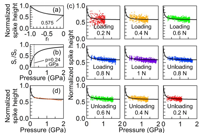
Figure 3 | Relating the ultrafast reflectivity changes to the pressure and real contact area. (a) Theoretical normalized spike height, \Psi_{r_j}(0, \tau_R) / \Psi(0, \tau_R) , plotted as a function of r_f . (b) Plot of the assumed variation of the ratio of the real to nominal contact area S_r/S_0 as a function of the pressure p , assuming the relation S_r/S_0 = p/(p + H) . The vertical dotted line represents the hardness H fitted from all our data. (c) Measured normalized spike-height vs calculated pressure p , obtained from the data of Fig. 2(c). The solid curves are fitted from theory, assuming H = 0.24 GPa. (d) Combined data (dotted curve) from the 9 plots in (c) together with theoretical fit (solid curve).
