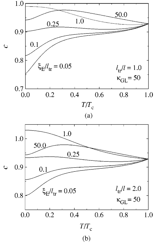
FIG. 8. The coefficient c(T) \equiv (1 - B/H_{c2})^{1/2} \Delta(T) / \Delta_0(B, T) in the extreme type-II case \kappa_{GL}=50 as a function of T/T_c for several values of \xi_E/l_{tr} . (a) l_{tr}/l=1.0 ; (b) l_{tr}/l=2.0 .
