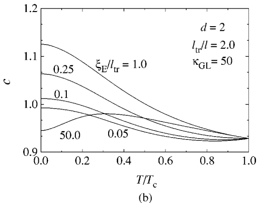
FIG. 10. The coefficient c(T) in two dimensions with \kappa_{GL}=50 as a function of T/T_c for several values of \xi_E/l_{tr} . (a) l_{tr}/l=1.0 ; (b) l_{tr}/l=2.0 .
