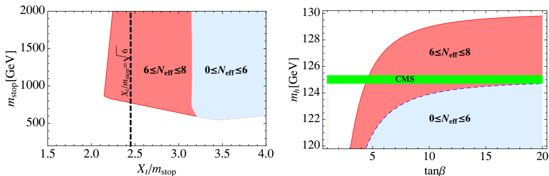
Figure 4. X_t/m_{\text{stop}} vs. m_{\text{stop}} and \tan\beta vs. the lightest Higgs mass in the case with (T_{\text{GUT}}, T_X) = (2 \times 10^{16} \text{ GeV}, 10^7 \text{ GeV}) and 0 \leq N_{\text{eff}} \leq 6 (light blue), 6 \leq N_{\text{eff}} \leq 8 (light red). The dashed line corresponds to X_t/m_{\text{stop}} = \sqrt{6} . In the right figure, m_h is calculated at the two-loop level using m_t = 172.9 \text{ GeV} , and m_{\text{stop}} is lighter than 2 TeV. The green band is the CMS result on Higgs mass from h \rightarrow \gamma\gamma, ZZ channels [47].
