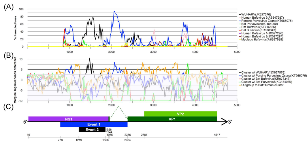
Figure 4. Recombination analyses of megabat bufavirus 1. Abscissae represent positions adjusted to reflect the position in the megabat bufavirus 1 genome. (A) Bootscan results supporting the clustering of megabat bufavirus 1 with other strains, which are color-coded as shown to the right. The ordinate shows the percentage of permuted trees supporting the clustering in each window. (B) Bayesian marginal likelihood support for the topological position of megabat bufavirus 1. The ordinate shows the log difference for the marginal likelihood of the model assuming the topological hypothesis and the model assuming the opposite. Lines below the threshold support ( <3 ) are shown as a lighter colour. (C) Genome representation showing the supported recombination events and the position relative to the protein encoding regions. Event 1 and Event 2 show the supported recombination events between MgBuV1 and porcine parvovirus Zsana or between MgBuV1 and WUHARV parvovirus, respectively. Nucleotide positions 778, 1219, 1856 and 2384 show putative recombination breakpoints.
