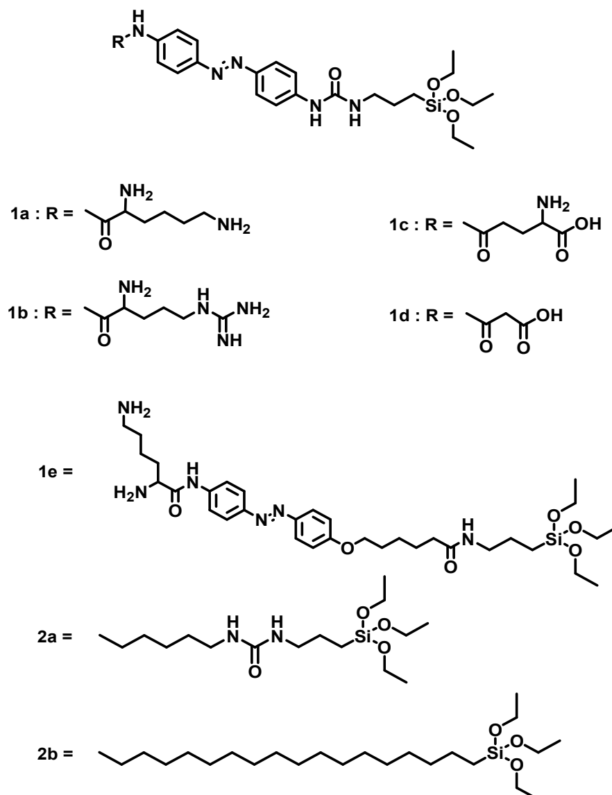
Chart 1 Chemical structure of photoresponsive azobenzene silane compound (1a-e) along with alkyl silane chain (2a and 2b).
