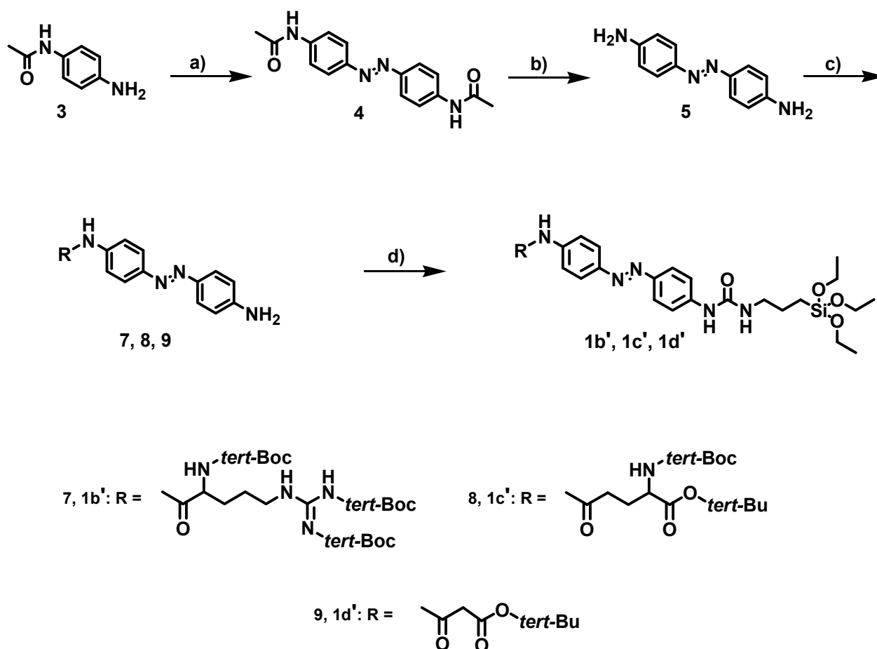
Scheme 1 a) NaBO 3 , H 3 BO 3 , HOAc, HCl, MeOH, 60 °C. b) NaOH. c) For 7, 1b' = Boc-Arg-(Boc) 2 -OH, for 8, 1c' = Boc-Glu-(OtBu)-OH and for 9, 1d' = Mono-tert-butyl malonate, DCC, HOBT, DMF. d) OCN-(CH 2 ) 3 -Si(OEt) 3 , THF.
