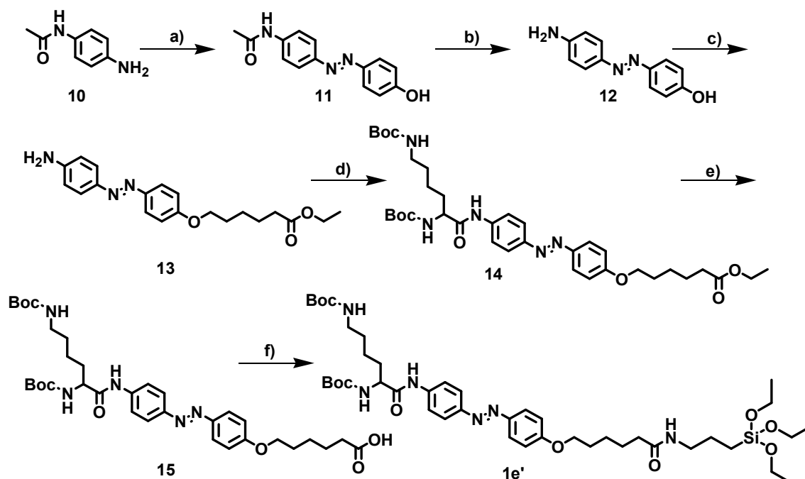
Scheme 2 a) HCl, H 2 O, NaNO 2 , NaOH, PhOH, 0–2 °C. b) 10% NaOH, Reflux 2h. c) Br-(CH 2 ) 5 -COOEt, K 2 CO 3 , (CH 3 ) 2 CO, 50–60 °C. d) Boc-Lys-(Boc)-OHL.DCHA, DCC, HOBt, DMF. e) Dioxane, 1M aq. KOH. f) OCN-(CH 2 ) 3 -Si-(OEt) 3 , THF.
