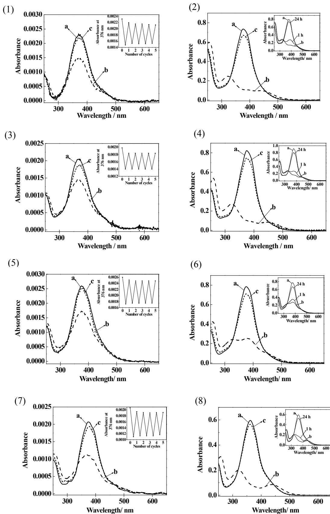
5 Fig. 1 Absorption spectral changes of 10% of 1b-e and 90% of 2a or 2b in quartz surface after deprotection of tert -Boc group [left (1), (3), (5), (7)] and that of 1b'-d' in acetonitrile and 1e' in DCM before deprotection of tert -Boc group [right (2), (4), (6), (8)]. (a) Before irradiation. (b) photostationary state
