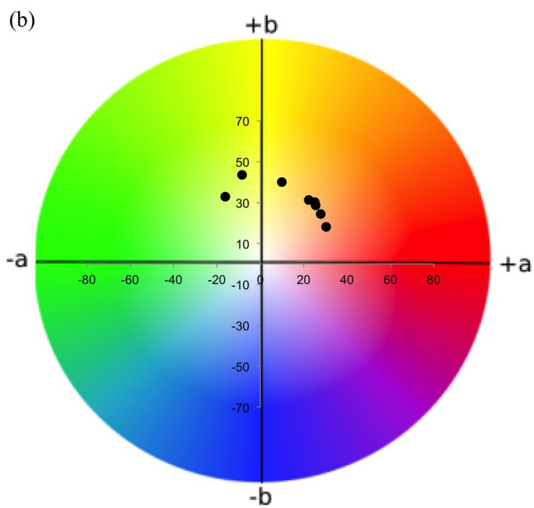
Fig. S3 (a) 3D and (b) 2D plot of various pH values in CIE L^*a^*b^* color system.
