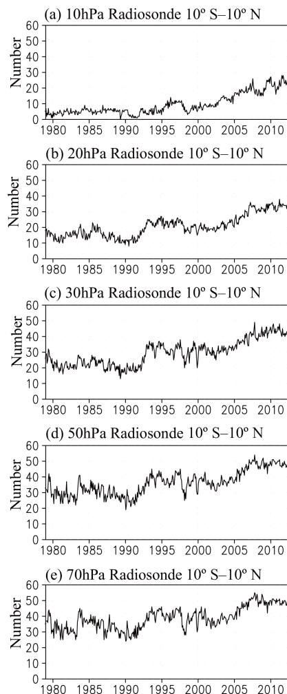
Figure 15. Time variation in number of radiosonde observations at 10^{\circ} S– 10^{\circ} N at (a) 10, (b) 20, (c) 30, (d) 50, and (e) 70 hPa from 1979 to 2012.
