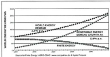
World Energy Scenario 2000 - 2050 Source for Finite Energy: ASPO-ODAC www.energypros.de & Kyoto Protocol 03 2636 2002
