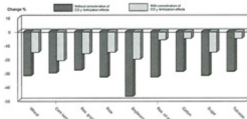
Global yield changes of plant products with and without consideration of CO 2 - fertilizer effects
