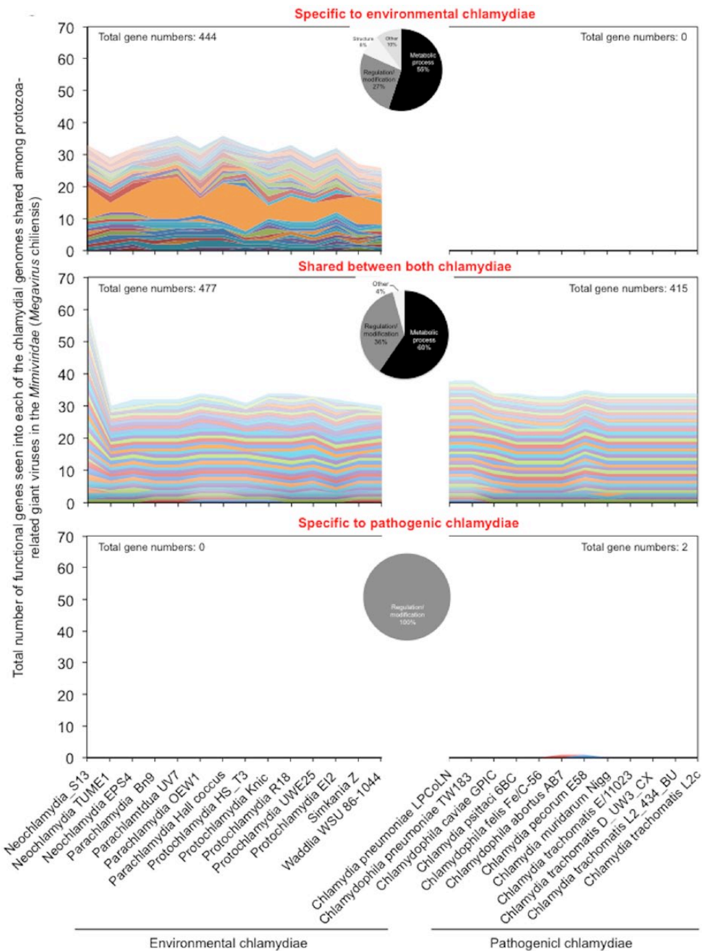
Figure 3. Total number of functional genes in each of the chlamydial genomes shared among protozoa-related giant viruses in the Mimiviridae ( Megavirus chilensis ). The genes shared between protozoa-related giant viruses in the Mimiviridae ( Megavirus chilensis ) and each of the chlamydiae were extracted, from a comparative genome analysis with RAST (see filter conditions into Material and Methods). Functional annotation was performed using the Kyoto Encyclopedia of Genes and Genomes (KEGG) 23 or the Universal Protein Resource (UniProt). 24 Upper panel: specific to environmental chlamydiae; Middle panel: shared between both chlamydiae; Lower panel: specific to pathogenic chlamydiae. Colors show distinct gene functions annotated by KEGG or UniProt. Pie charts in the center show the prevalence of genes classified into the categories of “Metabolic process,” “Regulation/modification,” “Structure,” and “Others.”
