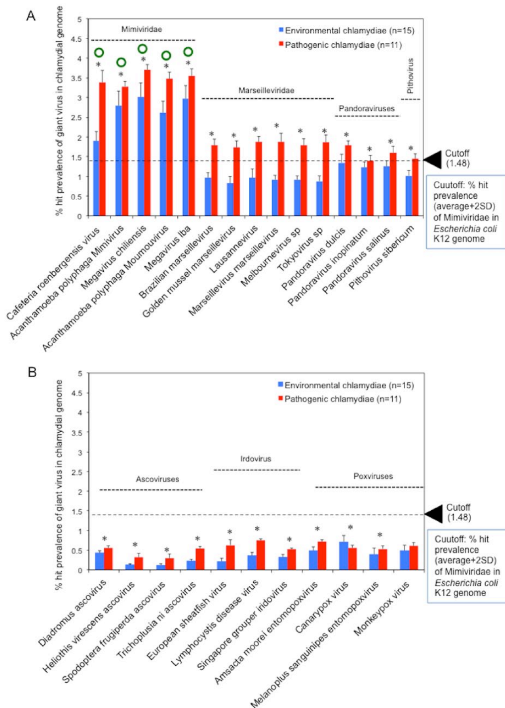
Figure 1. Comparisons of the prevalence rates of giant virus genes in chlamydial genomes and of the trend of dispersion on the prevalence of giant virus genes between pathogenic and environmental chlamydiae. Panels (A) and (B) show protozoa-related giant viruses and protozoa-unrelated giant viruses, respectively. Blue and red bars show the prevalence of giant virus genes in environmental and pathogenic chlamydial genomes, respectively. Comparisons of the prevalence rate were conducted using Mann–Whitney’s U test. Stars show a significant difference ( P < .05 ) between the prevalence values of environmental and pathogenic chlamydiae. Green circles show a significant difference in the prevalence rate of giant virus genes with values more than cut-off. Cut-off (1.48%) as a background value (dashed line) was defined by the prevalence of genes from Mimiviridae ( Cafeteria roenbergensis virus, Megavirus chilensis , Megavirus Iba , Mimivirus , Moutmouvirus ) in the Escherichia coli K12 genome ( 1.28 \pm 0.19\% ) (see Table S5).
