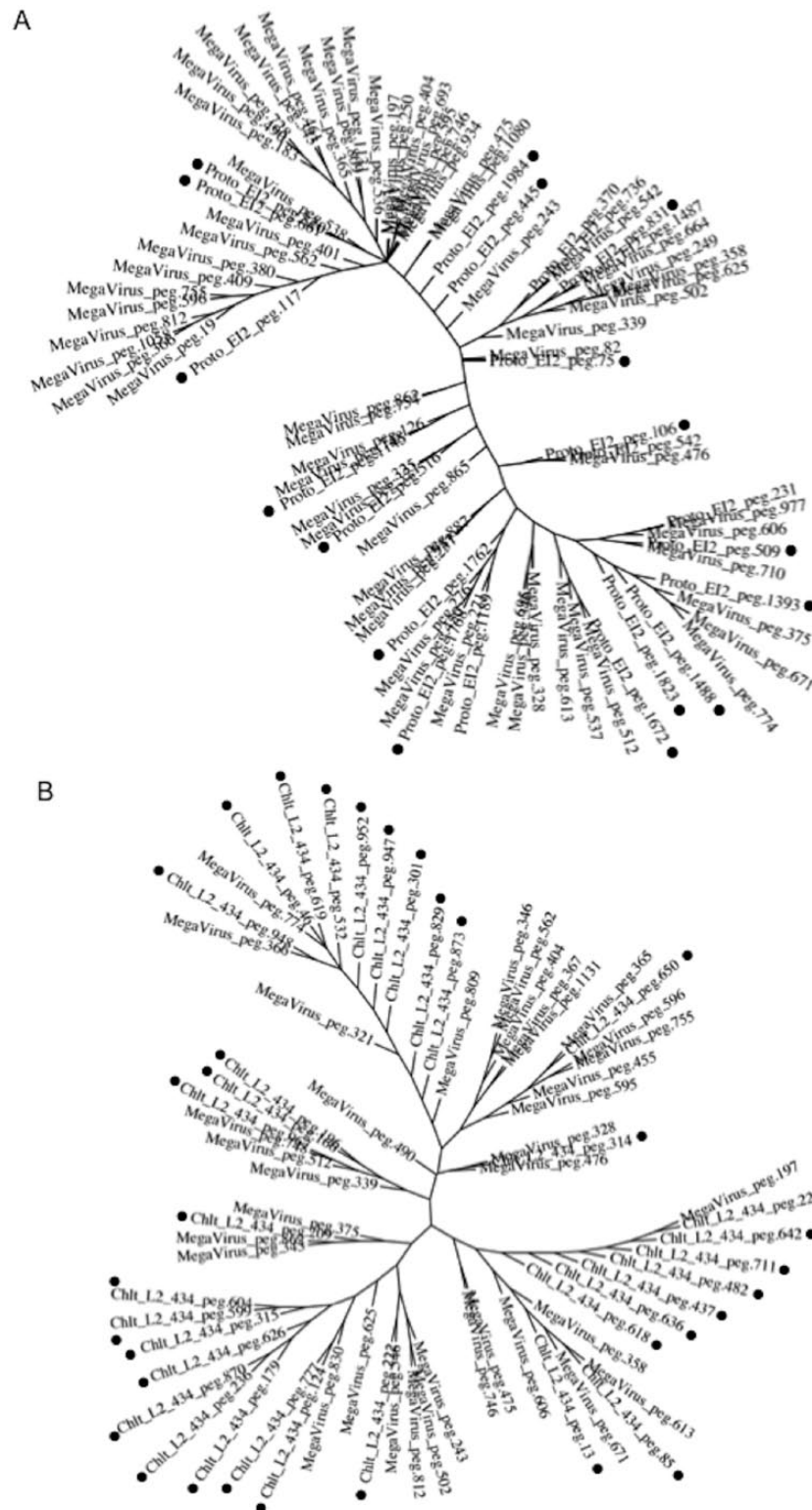
Figure 2. Phylogenetic analysis with most prevalent sets ( Megavirus chiliensis and Protochlamydia E12 or Chlamydia trachomatis L2 434Bu) showing several clusters. Trees (A) and (B) show Megavirus chiliensis (MegaVirus) with Protochlamydia E12 (Proto_E12) and with Chlamydia trachomatis L2 434Bu (Chlt_L2), respectively. Additional numbers (peg) show gene ID numbers assigned by RAST (see Table S1 to S4b). Black circles show these chlamydial genes. Phylogenetic trees were constructed with a maximum parsimony method by using MAFFT version 7 ( https://mafft.cbrc.jp/alignment/software/ ). 23
