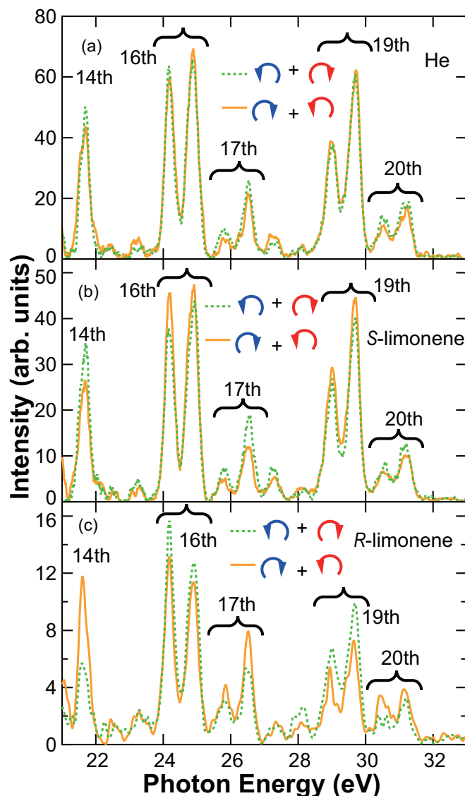
FIG. 2. High-order harmonics spectra from (a) He, (b) S -limonene, and (c) R -limonene, generated by the synthesized laser field by the CP \omega and 2\omega . The spectra shown by the green dotted (orange solid) lines have been generated by the combination of \omega and 2\omega , of which the rotational directions of the polarization are clockwise (counterclockwise), represented by a red arrow, and counterclockwise (clockwise), represented by a blue arrow, respectively.
