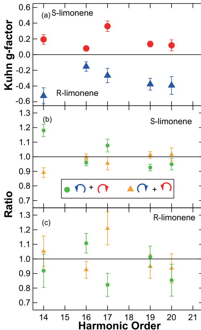
FIG. 3. (a) Kuhn g -factors from the enantiomers for each higher-order harmonic order. (b), (c) Intensity ratio of each high-order harmonic from limonene enantiomers and helium. The solid circles and triangles have been obtained by the clockwise and counterclockwise \omega in combination with the counter-rotating 2\omega , respectively.
