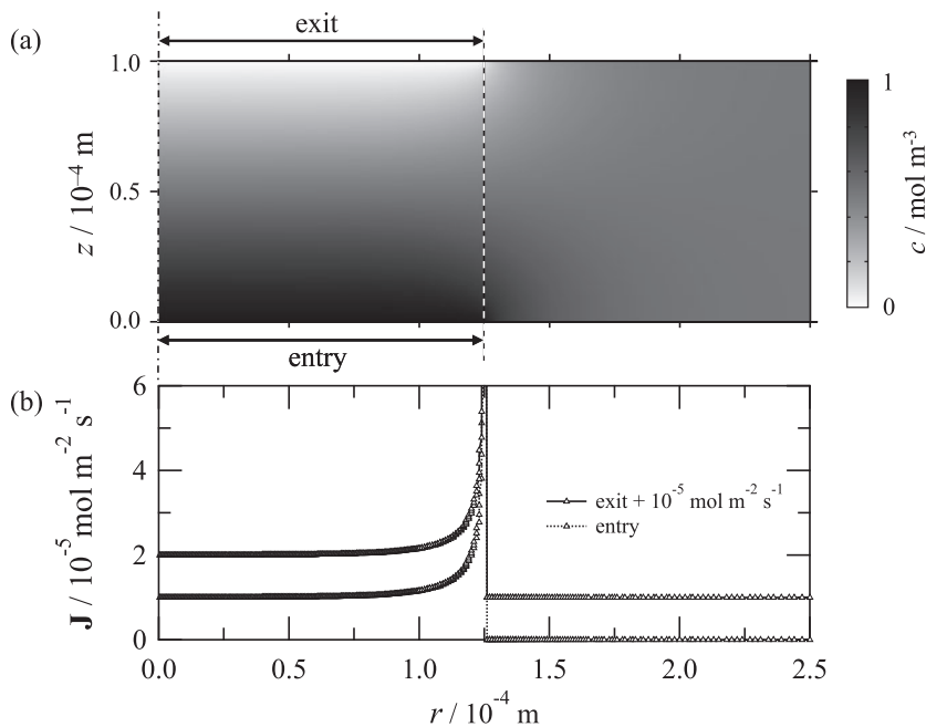
Fig. 5. (a) Cross-sectional distribution of hydrogen in the sheet and (b) local fluxes of the entry and exit sides during permeation measurement when both the entry and exit sides were 2.5 \times 10^{-4} m in diameter. The hydrogen diffusion coefficient of the sheet was 10^{-9} m 2 s -1 . In (b), the exit flux was shown with an offset of 10^{-5} mol m -2 s -1 .
