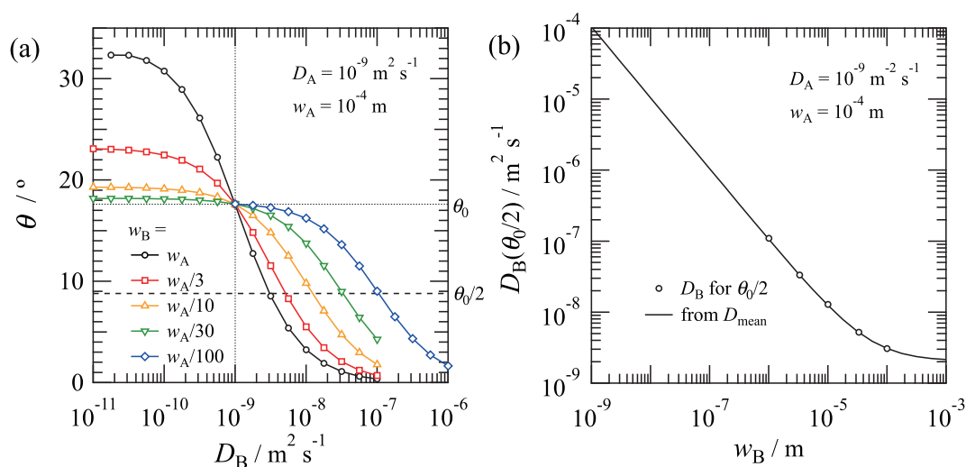
Fig. 7. (a) Relation between \theta and diffusion coefficient D_B of domain B in a heterogeneous sheet with L = w_A = 10^{-4} m, D_A = 10^{-9} m 2 s -1 , and f = 0.01 Hz when the width w_B of domain B was changed. (b) Plot of D_B(\theta_0/2) , showing a half of \theta_0 obtained in the homogeneous sheet, as a function of w_B . The relation calculated from Sekine 6) was also plotted as a solid line. (Online version in color.)
