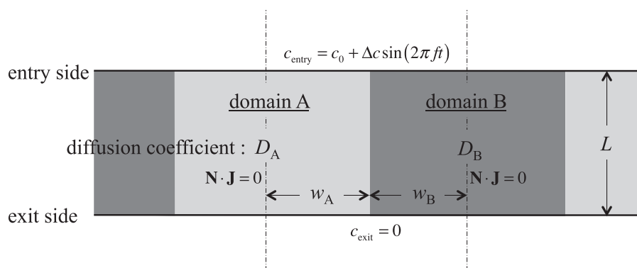
Fig. 6. Schematic diagrams of a heterogeneous sheet composed of domains used for a two-dimensional diffusion problem. Lamella of domains with different diffusivities was located perpendicularly with different width or thickness, respectively. A dotted line indicates the symmetric center of the domain for the periodic boundary condition of FEM calculation used.
