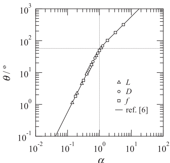
Fig. 2. Relations between \theta and \alpha when L , D or f was changed from default values of L = 10^{-4} \text{ m} , D = 10^{-9} \text{ m}^2 \text{ s}^{-1} and f = 0.01 \text{ Hz} . The relation reported by Sekine 6) was also plotted as a solid line. \alpha = (\pi f L^2 / D)^{1/2} .
