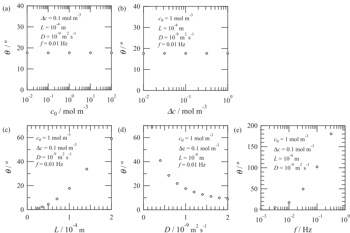
Fig. 1. Dependencies of phase shift \theta on (a) mean concentration c_0 and (b) concentration amplitude \Delta c of hydrogen at the entry side, (c) thickness L of the sample sheet, (d) diffusion coefficient D of hydrogen in the sheet and (e) frequency f of entry perturbation. The values of c_0 = 1 \text{ mol m}^{-3} , \Delta c = 0.1 \text{ mol m}^{-3} , L = 10^{-4} \text{ m} , D = 10^{-9} \text{ m}^2 \text{ s}^{-1} and f = 0.01 \text{ Hz} were used as default values.
