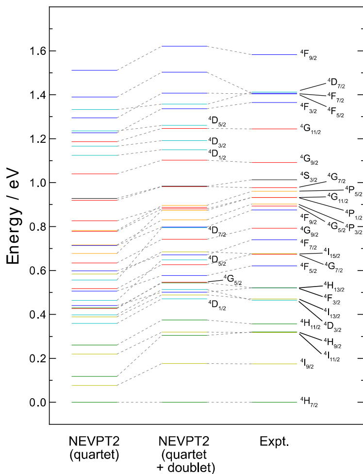
Figure 4. The NEVPT2 and experimental [11] energy levels of the ground and low-lying excited states of Ce + which originate from the ground-state configuration ([Xe]4f 1 5d 2 ). As for NEVPT2 results, two different calculated results are shown (SA-RASSCF/NEVPT2 for quartet and SA-CASSCF/NEVPT2 for quartet and doublet) where the energy levels in the left (NEVPT2 (quartet)) are the same as those of the middle one in Fig. 3a.
