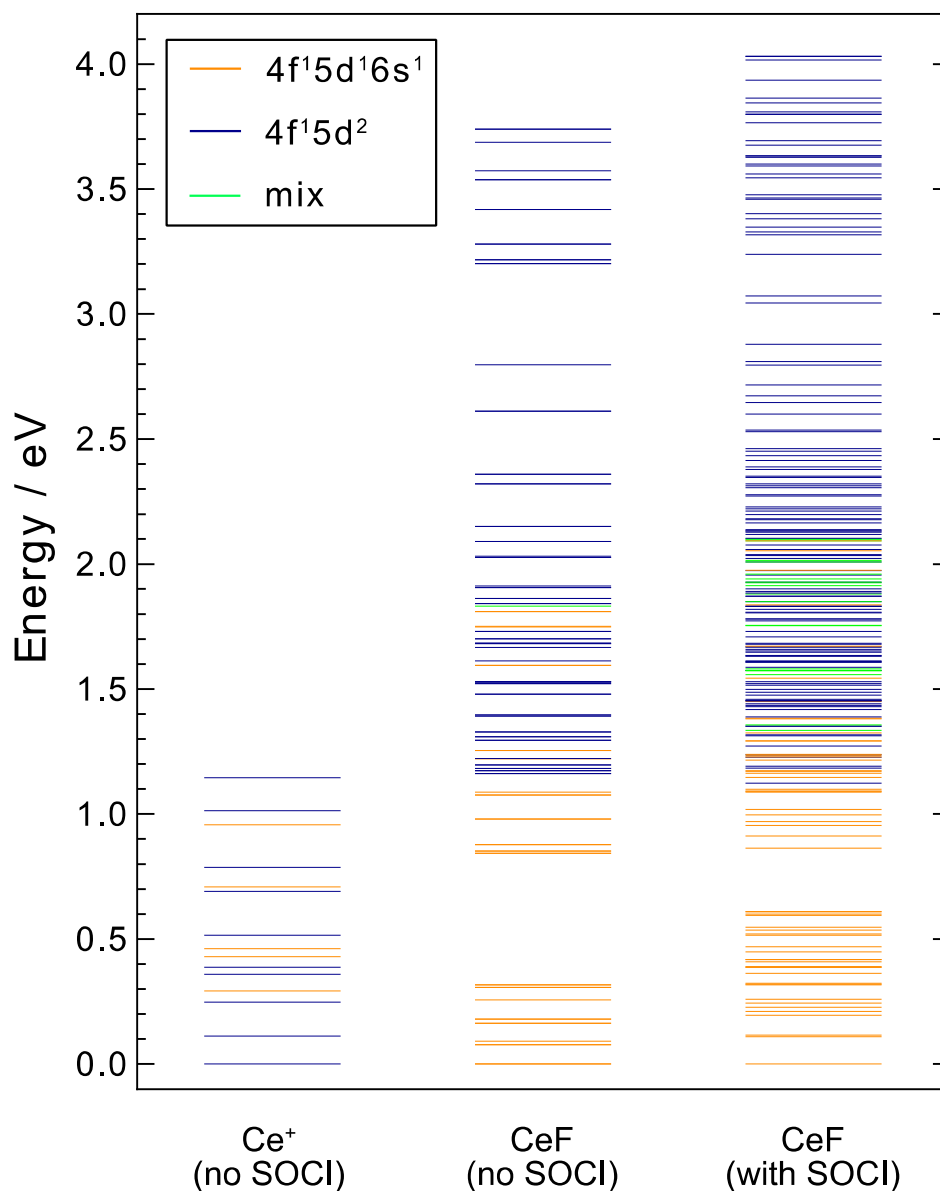
Figure 5. The energy levels of the low-lying electronic states of Ce + (without SOCI; the same as those in Fig. 2) and CeF (without and with SOCI), derived from the [Xe]4f 1 5d 1 6s 1 and [Xe]4f 1 5d 2 configurations of the Ce + part, calculated at the SA-RASSCF/NEVPT2 level with the Sapporo-QZP basis sets. The calculations for CeF were performed at the experimental bond length, r(\text{Ce-F}) = 2.048 \text{ \AA} . [36]
