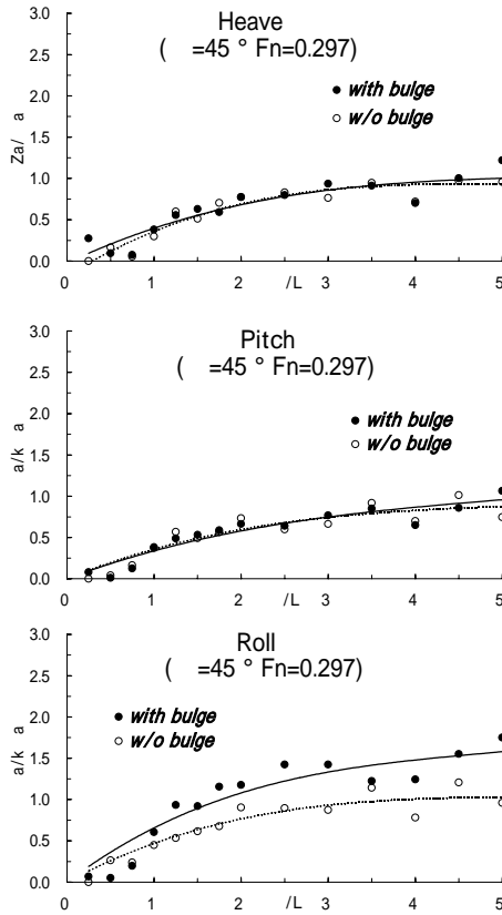
Fig.7 Measured motions in quartering waves (Fn=0.297, lines denote mean value of exp.)
