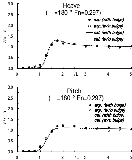
Fig.4 Heave and pitch in head waves ( Fn=0.297 )
