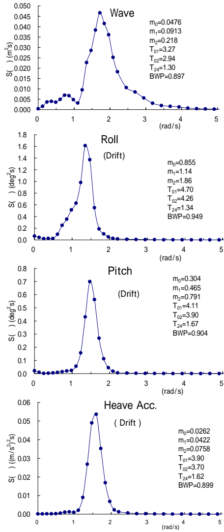
Fig.10 Measured motion spectra (drift condition)
