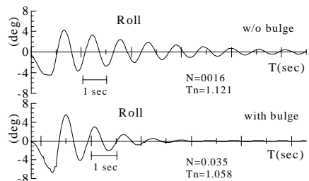
Fig.6 Roll measured from free decay tests ( Fn=0 )
