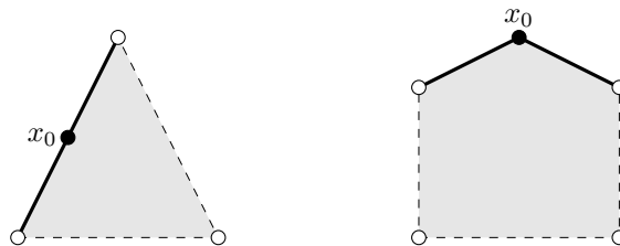
FIGURE 2. P_{x_0} .
