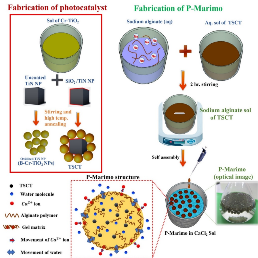
Figure 1. Schematic representation of TiN/ \text{SiO}_2 / \text{Cr-TiO}_2 (TSCT) and B-Cr- \text{TiO}_2 nanostructure fabrication using with and without \text{SiO}_2 cladded TiN NPs, respectively. Fabrication of TSCT P-Marimo structure is also shown.
