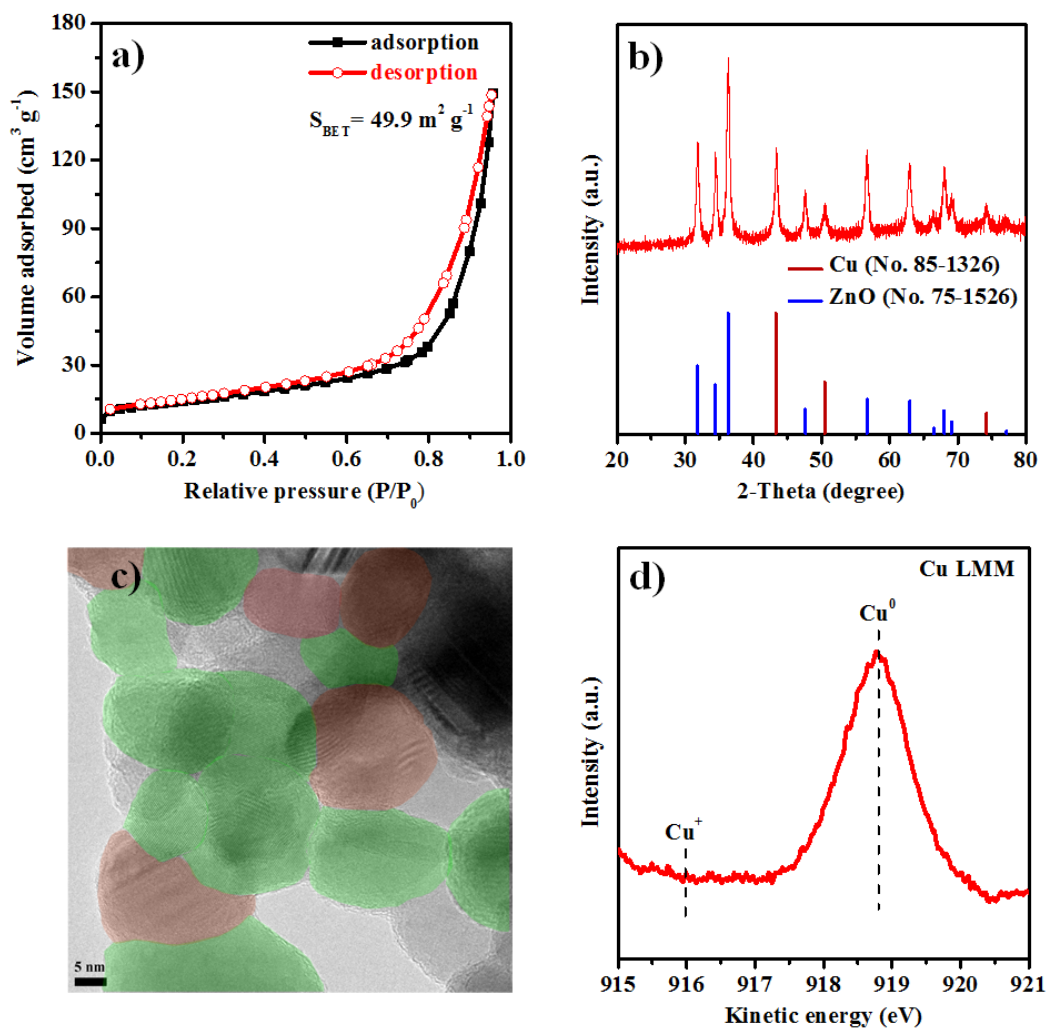
Fig. 1. Physicochemical characterizations of the reduced Cu/ZnO catalyst. (a) N 2 sorption isotherms; (b) XRD patterns; (c) HR-TEM image with Cu 0 in reddish brown and ZnO in light green; (d) Cu LMM AES spectrum.
