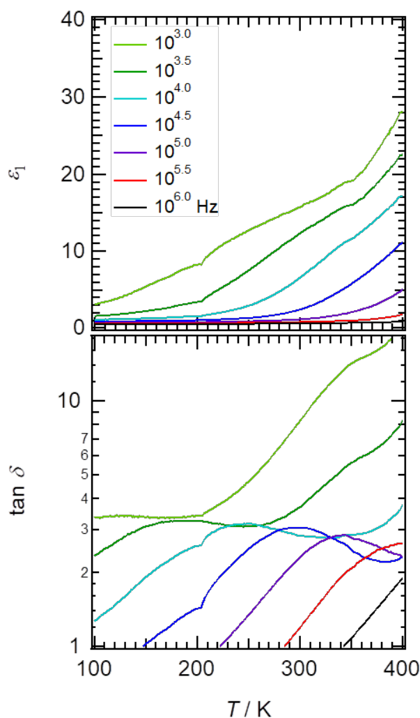
Figure 5 Temperature and frequency dependence of the real part of the dielectric constant ( \epsilon_1 ) and the dielectric loss tangent ( \tan \delta ) of crystal 4 .
