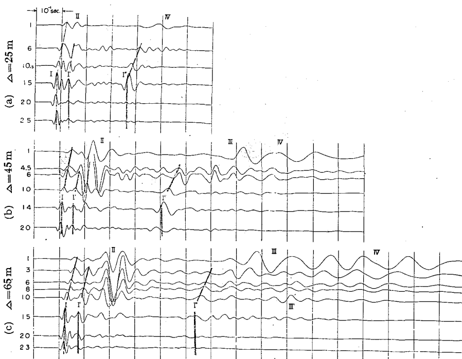
Fig. 9. (a) Seismic records at 25 m distance from shot hole. (b) Seismic records at 45 m distance from shot hole. (c) Seismic records at 65 m distance from shot hole.
