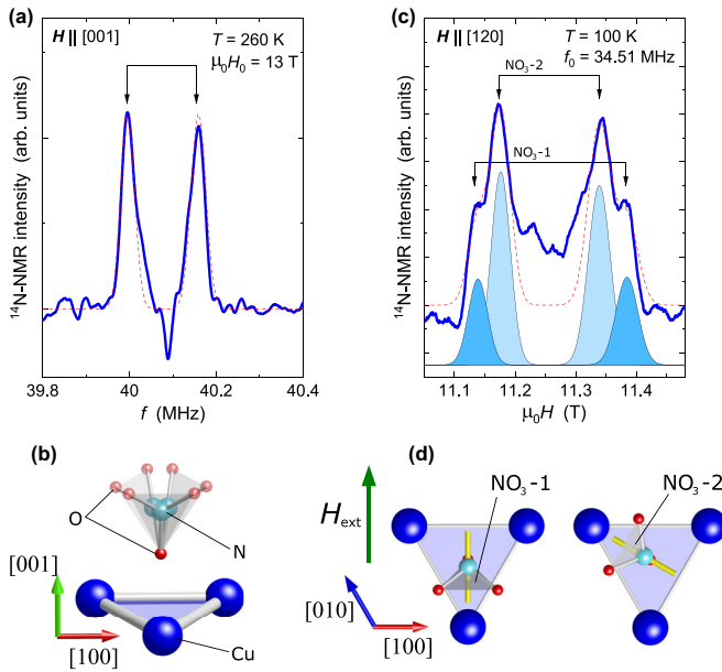
FIG. 3. ^{14}\text{N} -nuclear magnetic resonance (NMR) spectra for single-crystalline CdK at high temperatures measured in (a) \mathbf{H} \parallel [001] and (c) \mathbf{H} \parallel [120] . Two-peak structure typical for I = 1 nuclear spin is observed in (a), while four peaks were observed in (c) because of the positional disorder of \text{NO}_3 ions. The shadowed four peaks are the result of spectrum simulation (see text for details). The sum of these four peaks is represented by the red dotted line. (b) Positional disorder of \text{NO}_3 ions located on a Cu triangle. Three possible \text{NO}_3 sites are randomly occupied. (d) In-plane structure of \text{NO}_3 ions. The orientation of the main principal axis of the electric field gradient (EFG) is indicated by a bar on the N sites. When the external field H_{\text{ext}} is applied along the [120] direction, N sites at \text{NO}_3 -1 and \text{NO}_3 -2 show different quadrupolar splitting.
