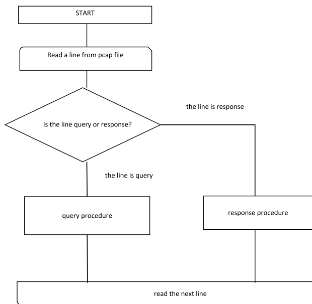
Fig. 8 The workflow of NS_DB creation program.
