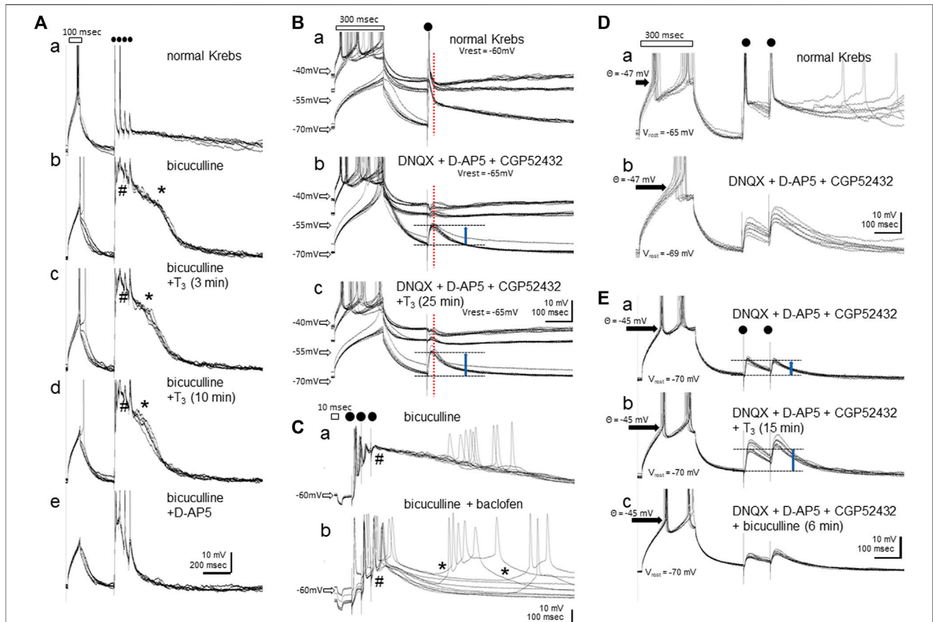
FIGURE 5 | Effects of bath-applied T_3 ( 40 \mu\text{M} ) on the membrane potentials in IMM neurons. (A–C) show recordings using normal \text{Cl}^- pipette solution. (D,E) show recordings with high- \text{Cl}^- electrode and GABA-A responses revealed as depolarization. (Aa–e) T_3 suppressed the NMDA-plateau. Initial depolarizing current injection (indicated by a rectangle, 100 msec) was followed by four repetitive local electric shocks (dots); # indicates the initial onset phase of the NMDA plateau potential by bicuculline, and * the shoulder (onset of the decaying phase) of it. Six consecutive traces recorded at 10 s intervals are shown for each. (Ba–c) Responses recorded at three steps of tonic current injection through the recording electrode. Vertical dashed red line indicates the peak GABA-A response that is reversed at ca. -50 \text{ mV} . V_{\text{rest}} means the resting membrane potential without current injection. (Ca–b) Baclofen induced sporadic NMDA-plateau depolarization (*). (Da–b) Blockade of AMPA, NMDA and GABA-B receptors unmasked GABA-A receptor mediated depolarization. (Ea–c) Further addition of T_3 enhanced the GABA-A depolarization (upward blue arrows). No effects were found in the resting membrane potential ( V_{\text{rest}} = -70 \text{ mV} ), membrane resistance, or threshold for spike generation ( \theta = -45 \text{ mV} ).
