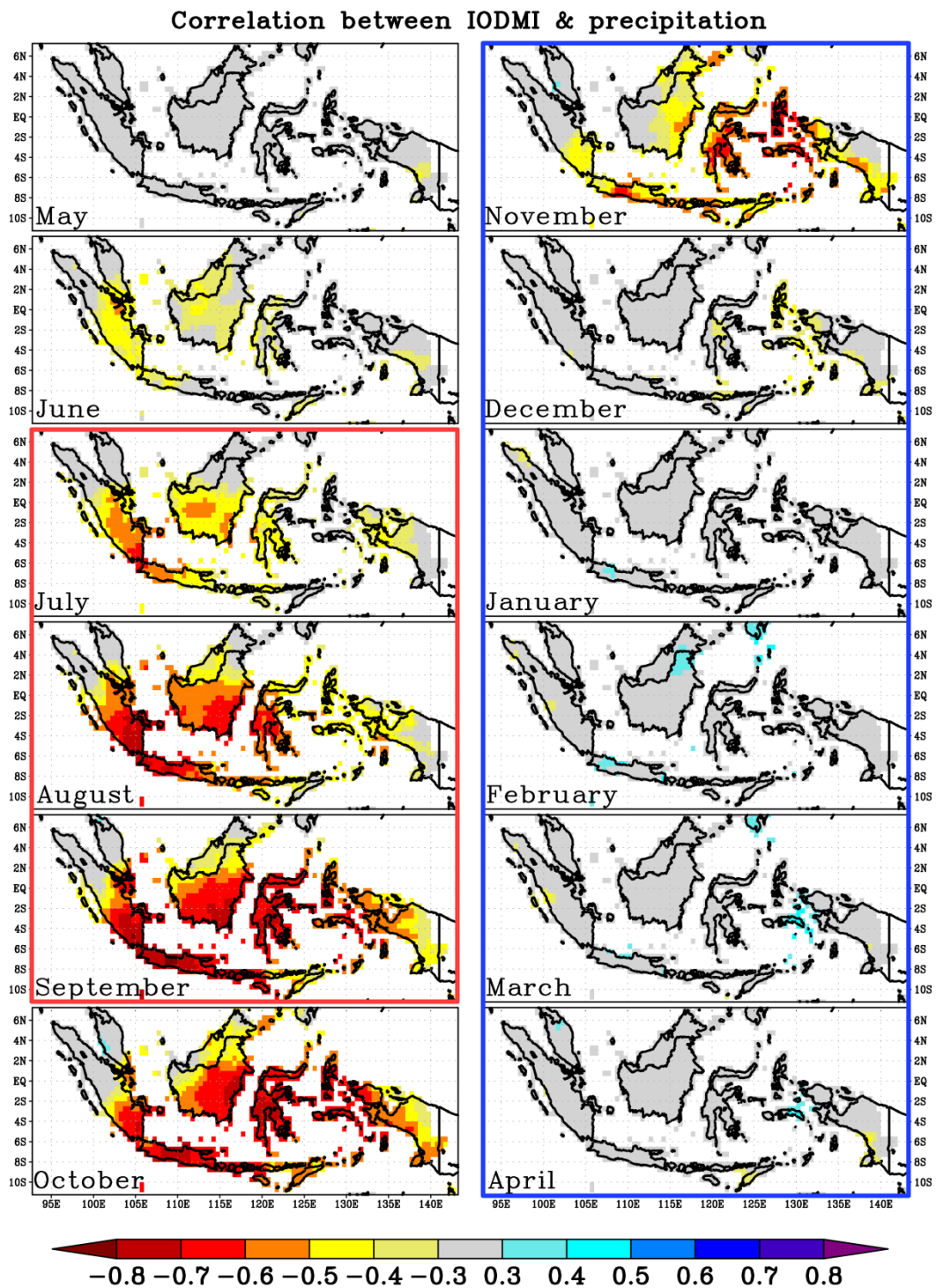
Figure 2.15. Spatial distribution of correlation coefficients of the seasonal development of the precipitation with normalized IODMI. Correlations are calculated for 3-month averaged data, and the center month is written in each panel. Only correlations that are significant at the 95% confidence level are shown by the color shading. Red and blue frames indicate the dry and wet seasons, respectively.
