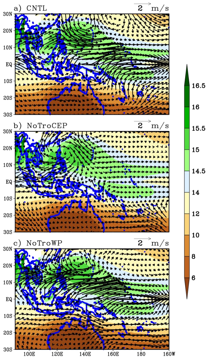
Fig. 3.7. JASO-mean 925 hPa climatological specific humidity (shading; \text{g kg}^{-1} ) and anomalous horizontal wind (vector) regressed onto normalized Niño-3.4 index for (a) CNTL, (b) NoTroCEP, and (c) NoTroWP. The wind scale is given by the arrows at the top right corner.
