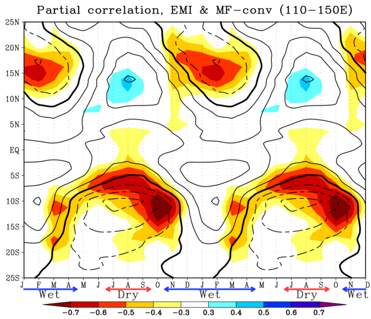
Figure 2.14. As in Fig. 2.9, but for EMI.
