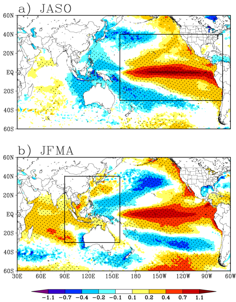
Fig. 3.2. Spatial distribution of anomalous SST ( ^{\circ}\text{C} ) regressed against normalized Niño-3.4 index for (a) JASO and (b) JFMA season with use of the OISST data. Dots denote the values that are significant at the 95% confidence level. Geographic location in (a) and (b) represents the tropical central-eastern Pacific (CEP) and western Pacific (WP), respectively.
