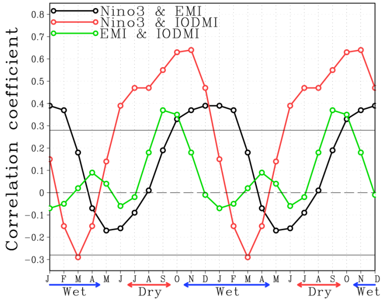
Figure 2.4. Correlation coefficients among SST-based climate indices with the 3-month average as a function of calendar month. The values outside the solid lines are statistically significant at the 95% confidence level. Red and blue arrows indicate the dry and wet seasons, respectively. The x axis indicates the center month of the 3-month average.
