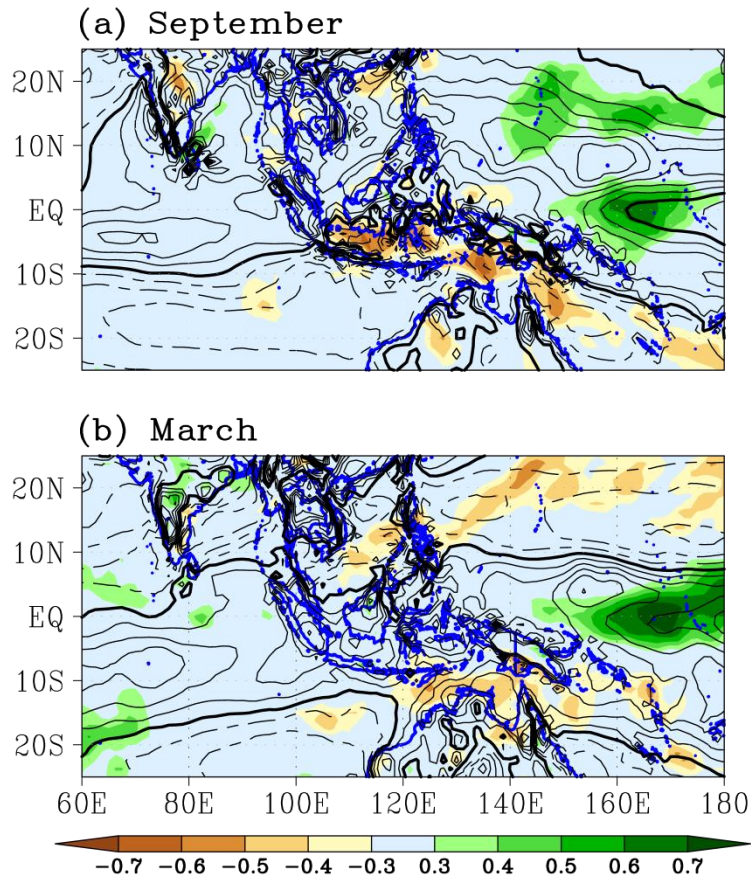
Figure 2.13. As in Fig. 2.8, but for EMI.
