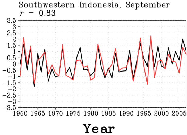
Figure 2.17. Time series of normalized IODMI and normalized and sign-reversed precipitation averaged over the area in Fig. 2.16, namely, the rectangular area in southwestern Indonesia ( 100^{\circ} – 113^{\circ} E, 10^{\circ} – 2^{\circ} S) between August and October. The center month of the 3-month average is shown in the panel title for consistency with other figures.
