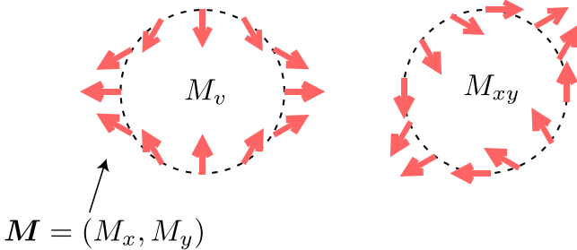
FIG. 8. Antivortex configurations of the magnetic dipoles \mathbf{M} = (M_x, M_y, 0) . The left and right panels show the different components of the magnetic quadrupoles, M_v and M_{xy} , respectively.
