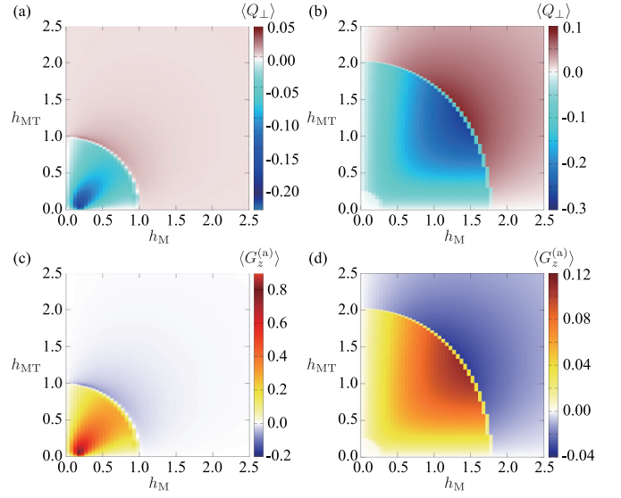
FIG. 6. Contour plots of (a), (b) \langle Q_\perp \rangle and (c), (d) \langle G_z^{(a)} \rangle in the plane of h_M and h_{MT} at (a), (c) \lambda = 0.5 and (b), (d) \lambda = 5 in the single-site system. The other model parameters are chosen at V_{sp} = 1 and \mu = 0 .
