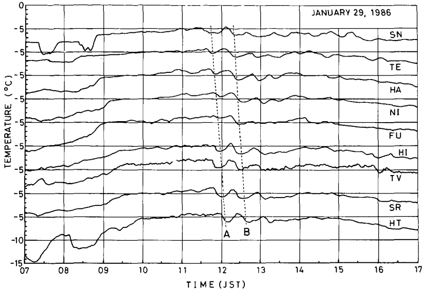
Fig. 2 Time series of temperature change at 9 observation points for the period 0700-1700 JST 29 January 1986.
