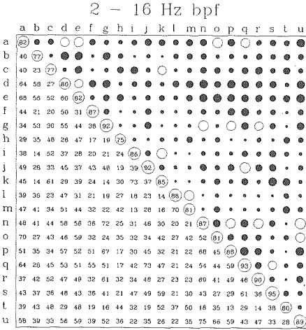
Fig. 5. Cross-correlation score for the earthquake families 'a' to 'u'. The mean of the maximum cross-correlations for all possible pairs of two set of the families is displayed corresponding to its position in the matrix. The cross-correlations are calculated by using the 2-16 Hz bandpass filtered seismograms. The circle size (upper-right half) is proportional to the cross-correlation values which are shown in the lower-left half in percent. Open circles in the upper-right half represent the correlation values greater than 0.6.
