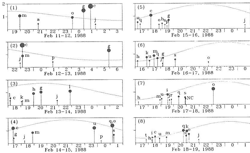
Fig. 8. Detailed time sequence of the earthquake occurrence in the eight burstic activities after the M 2.5 high-frequency event. The smooth curve indicates the vertical component of the solid earth tide. Family names of each event are attached. No systematic order of the family occurrence is recognized.
