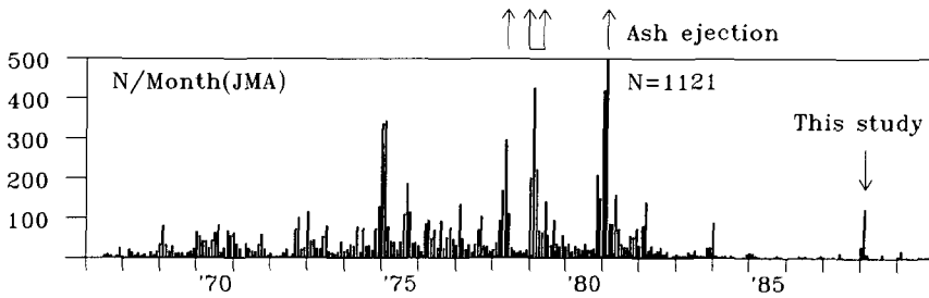
Fig. 2. Monthly frequency of volcanic earthquakes at Tarumai volcano observed by Japan Meteorological Agency (JMA).
