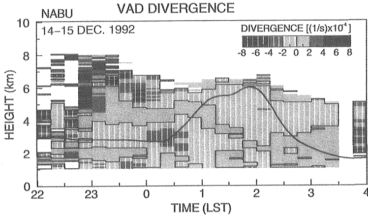
Fig. 8. The time-height cross section of the divergence profiles of the X-band Doppler radar at Nabu analyzed with the EVAD method from 2200 LST 14 December to 0400 LST 15 December 1992. The solid line shows the same boundary as in Fig. 7b.
