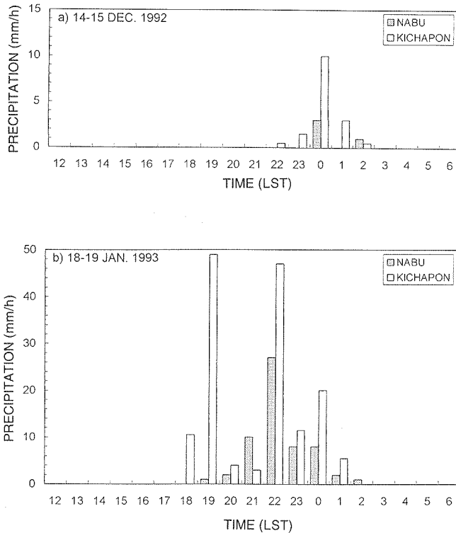
Fig. 3. The time series of precipitation at Nabu and Kichapon, (a) from 1200 LST 14 December to 0600 LST 15 December 1992 and (b) from 1200 LST 18 January to 0600 LST 19 January 1993.
