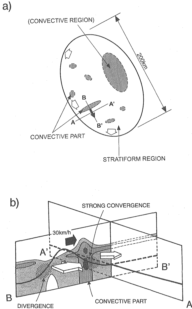
Fig. 14. The conceptual model of Case A. (a) The horizontal model of the cloud cluster. Shaded areas are observed (solid) and inferred (dashed) convective region. White arrows show growth of the cluster and the black arrow shows the direction of a convective echo that passed over Nabu. (b) Vertical model along A-A' and B-B' lines in Fig. 14a as a bird's-eye view from west in the observed area by the X-band radars. Shaded area is the radar echo, and the dotted area is the region of convergence and divergence. White arrows show the horizontal winds of the two layers and black arrow shows the direction of a convective echo and the wave.
