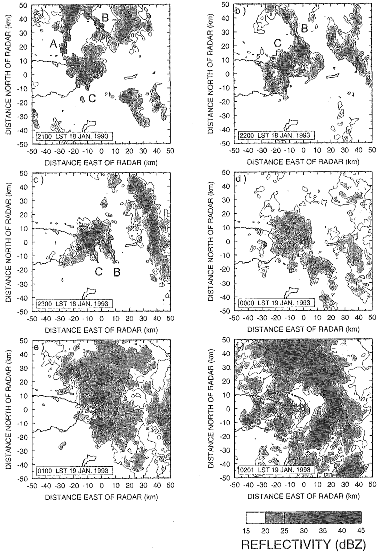
Fig. 13. Sequential horizontal cross sections of the reflectivity displays at the height of 3 km from ILTS radar every 1 hour from 2100 LST 18 to 0200 LST 19 January 1993. The reflectivity contour interval is 5 dBZ beginning at 15 dBZ. Convective linear echoes are labeled by A, B and C.
