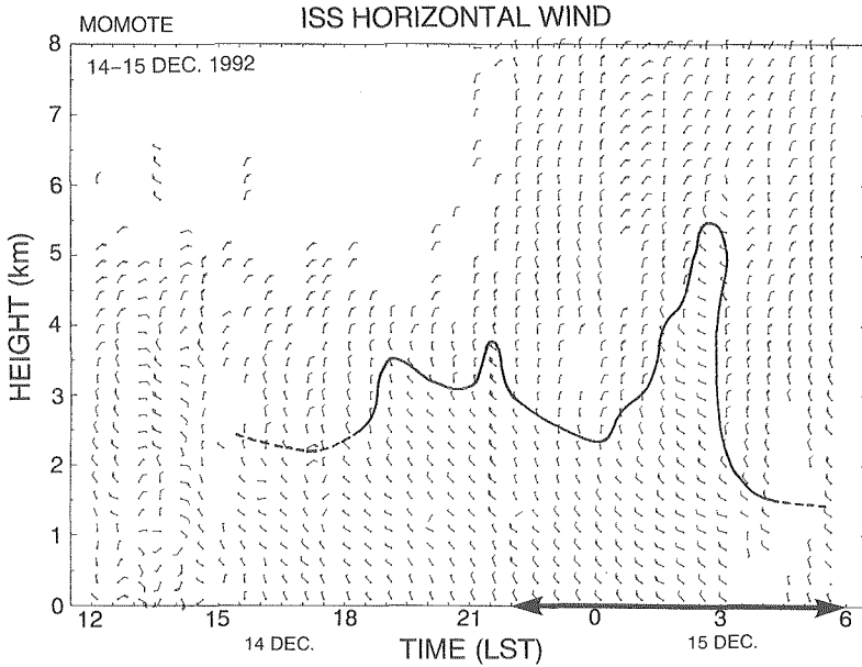
Fig. 5. The time-height cross section of horizontal wind profiles of the ISS radar at Momote from 1200 LST 14 December 1992 to 0600 LST 15 December 1992 (flag, 20 m/s; full barb, 5 m/s; and half barb, 2.5 m/s, respectively). The solid (dashed) lines show large (small) vertical shear of the horizontal wind. A solid line with arrows from 2200 LST 14 December to 0600 LST 15 December 1992 indicates the period of VAD and EVAD analyses with two X-band Doppler radars (see Fig. 7 and 8).
