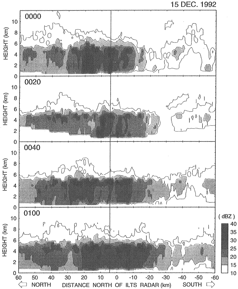
Fig. 10. Vertical cross sections of the reflectivity displays of X-band radar at Momote every 20 minutes from 0000 to 0100 LST 15 December 1992. The reflectivity contour interval is 5 dBZ beginning at 15 dBZ. Locations of these sections are indicated by the line A-A' in Fig. 9.
