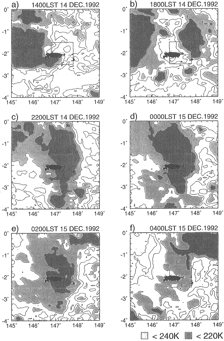
Fig. 2. The brightness temperature of the GMS-IR (at the interval 20 K) from 1400 LST 14 December to 0400 LST 15 December 1992. The black area shows Manus Island, and the shaded areas show T_{BB} less than 220 K. The rectangle represents the area in the X-band radar analysis of Fig. 6.
