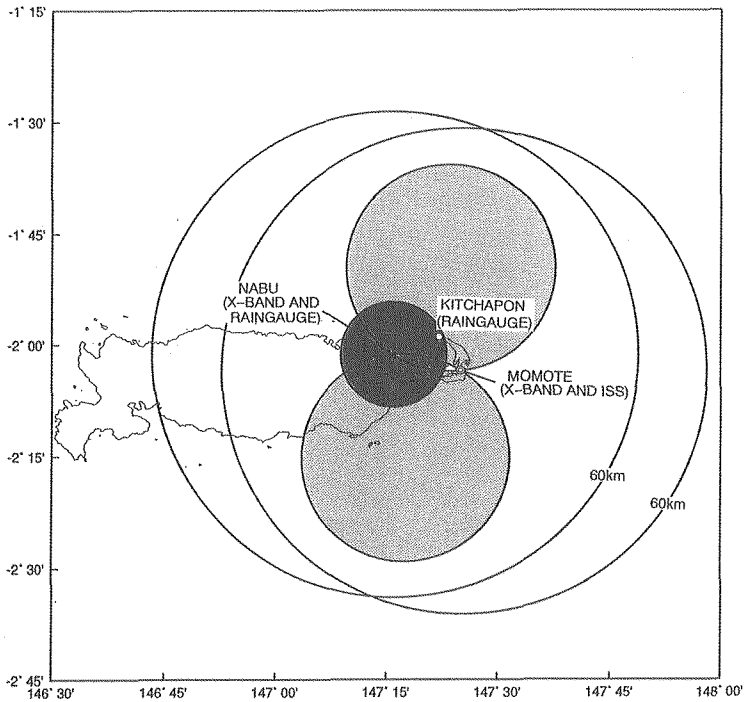
Fig. 1. Locations of an ISS, two X-band Doppler radars and two raingauges. The area analyzed by dual Doppler radar is lightly hatched. VAD and EVAD analysis ranges at an altitude of 5 km is shown by a dark circle.
