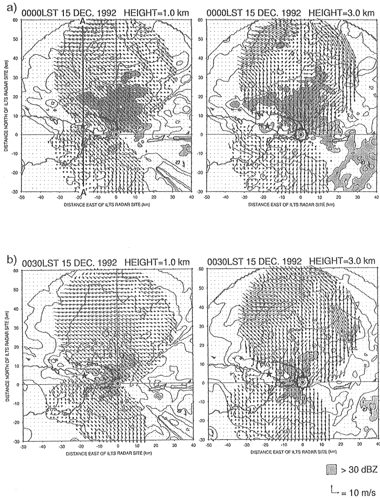
Fig. 9. The reflectivity of the X-band radar at Momote and the horizontal wind from the dual Doppler radar analysis at (a) 0000 LST and (b) 0030 LST 15 December 1992. The horizontal cross sections at 1.0 km (left) and 3.0 km (right) are shown. The reflectivity contour interval is 5 dBZ from 10 to 45 dBZ. The hatched area is greater than 30 dBZ. The double circles indicate Momote; the black star, Nabu.
