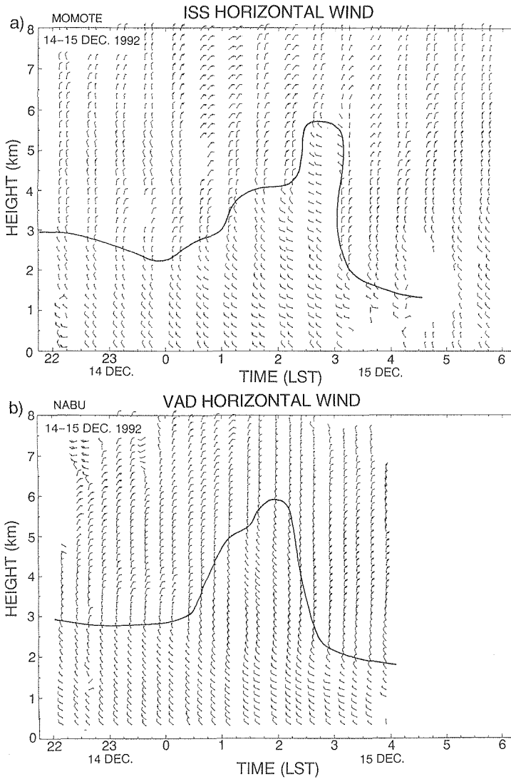
Fig. 7. The time-height cross section of the horizontal wind profiles of (a) ISS radar at Momote and (b) X-band Doppler radar at Nabu from 2200 LST 14 December to 0600 LST 15 December 1992. The flag and barbs represent the same values as in Fig. 5. The solid lines show a boundary between northwesterly wind and northerly wind.
