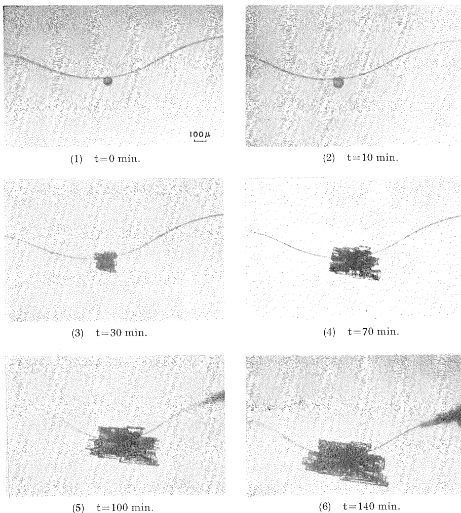
Fig. 9 A series of microphotographs of "hollow prisms" growing from a frozen droplet on rabbit hair.
