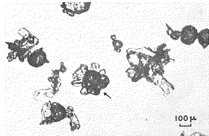
Fig. 5 Microphotograph of "frozen cloud droplets" taken at Syowa Station, Antarctica. The crystal indicated by arrow is a germ of radiating assemblage of plates growing from a frozen cloud droplet.
