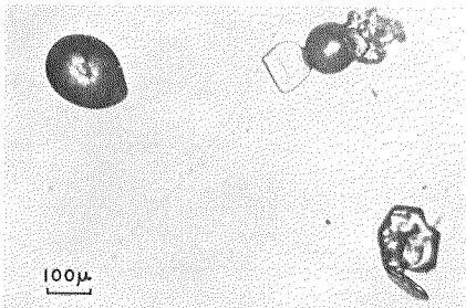
Fig. 4 Microphotograph of "frozen cloud droplets" taken at Syowa Station, Antarctica.
