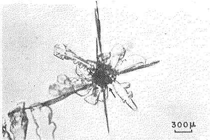
Fig. 2 Microphotograph of "radiating assemblage of dendrites" taken at Syowa Station, Antarctica.
