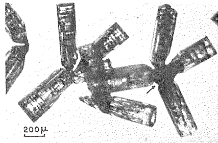
Fig. 3 Microphotograph of "combination of bullets" taken at Syowa Station, Antarctica.
