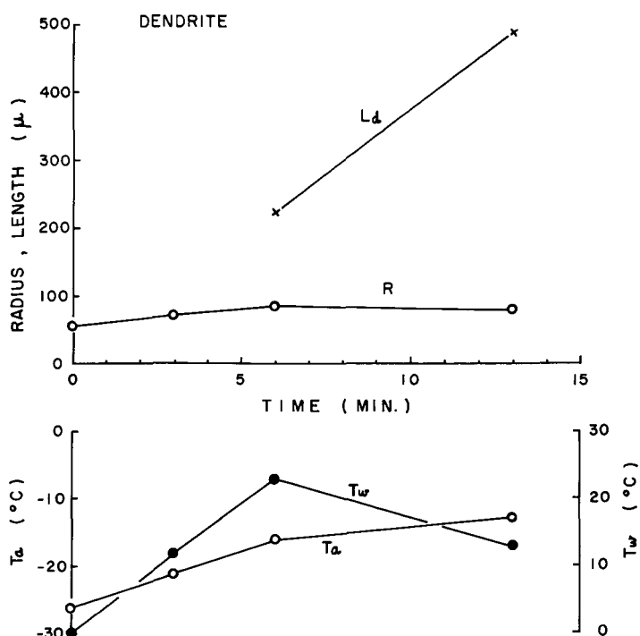
Fig. 7 Time changes of length of crystal ( L_d ) and radius of center frozen cloud particle ( R ) (upper) and T_a and T_w in the convection chamber (lower).
