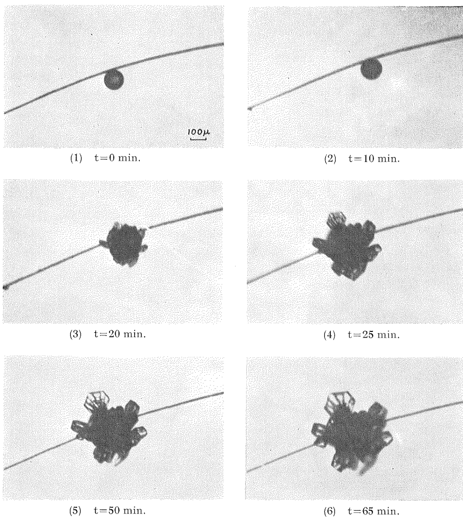
Fig. 8 A series of microphotographs of "radiating assemblage of plates" growing from frozen droplets on rabbit hair.
