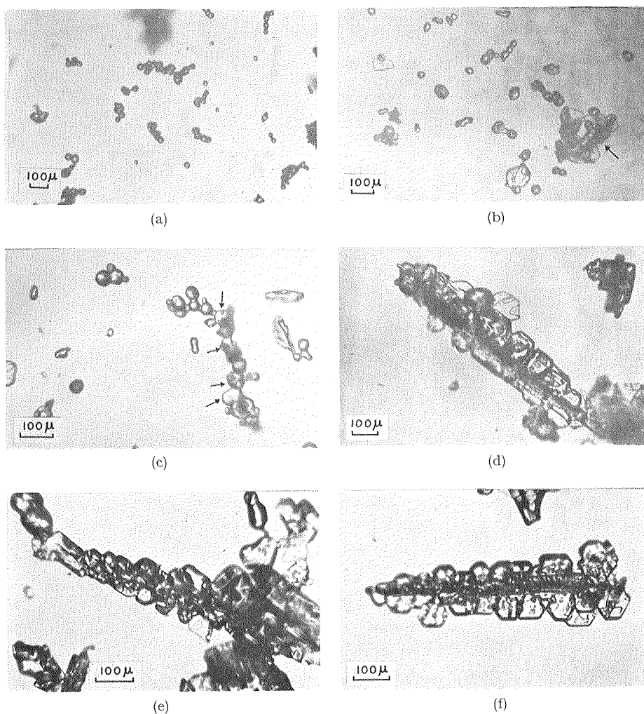
Fig. 1 Microphotographs of various stages from "sintered frozen cloud particles" to "scalelike side planes" taken at Syowa Station, Antarctica.
