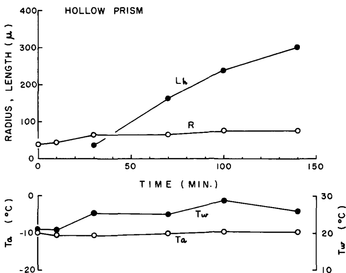
Fig. 10 Time changes of length of crystal ( L_h ) and radius of center frozen cloud particle ( R ) (upper) and T_a and T_w in the convection chamber (lower).
