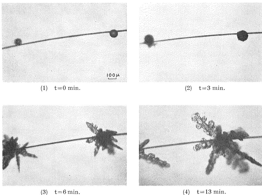
Fig. 6 A series of microphotographs of "radiating assemblage of dendrites" growing from frozen droplets on rabbit hair.
