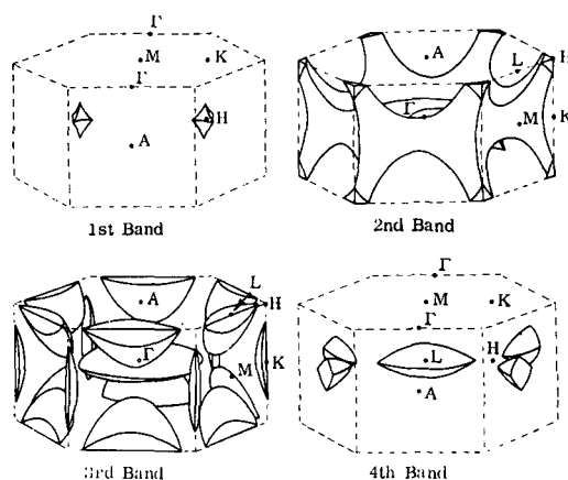
Fig. 8 The one OPW Fermi surface in the reduced zone scheme (after Harrison 1966).
