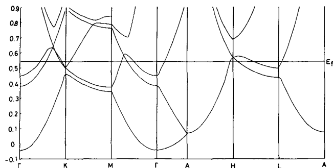
Fig. 4 The band structure corresponding to V/V_0=0.8 .
