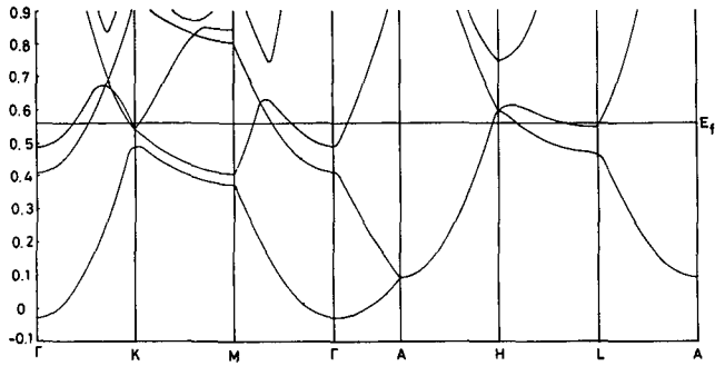
Fig. 5 The band structure corresponding to V/V_0=0.75 . The electrical resistance shows a maximum at this compressed state.
