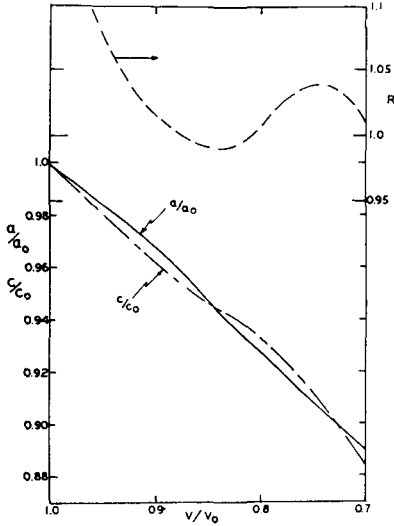
Fig. 10 The variations of a/a_0 , c/c_0 and the resistance versus V/V_0 for magnesium. (after Drickamer)
