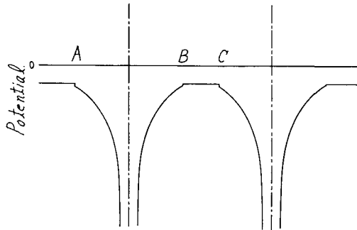
Fig. 1 The illustrative muffin tin potential for one dimensional lattice.
