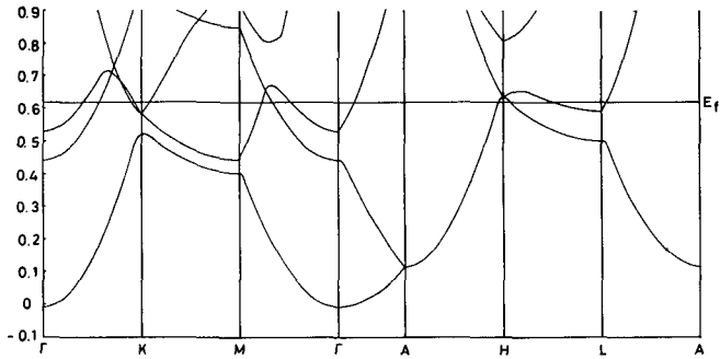
Fig. 6 The band structure corresponding to V/V_0=0.7 . It is seen that the electronic structure almost recovers to that of the normal state.
