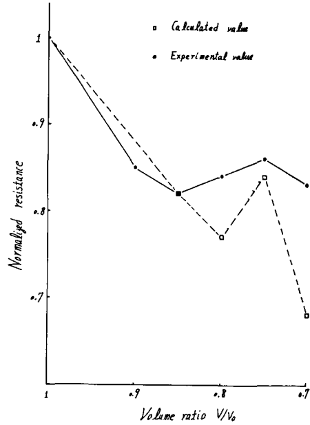
Fig. 11 The calculated and the experimental resistances which are normalized by the values of the normal state. The experimental values are referred from the figure 10.
