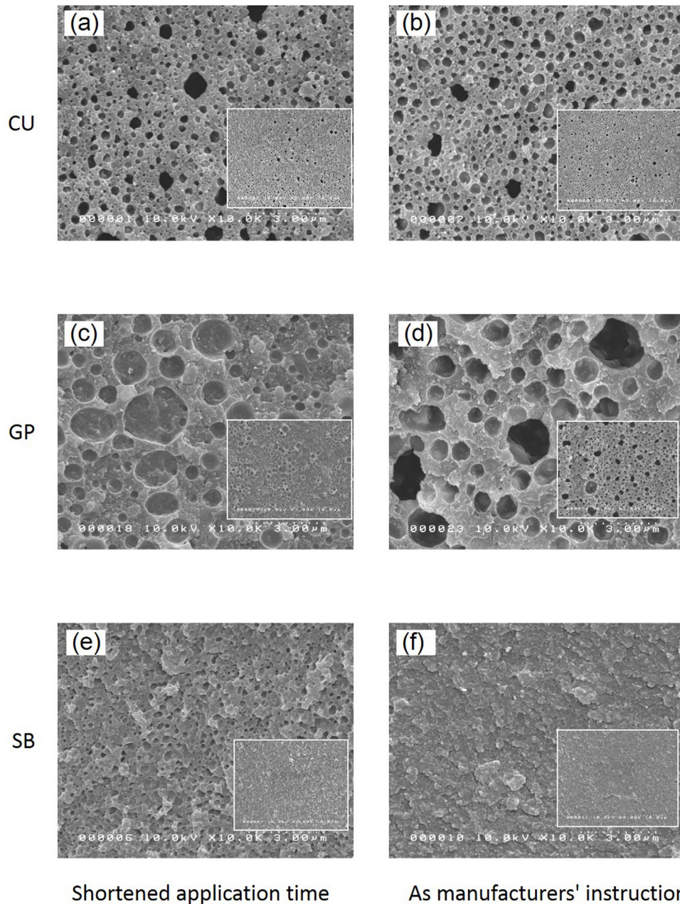
Fig. 2. Representative SEM images of failure mode in bur-cut dentine group at high magnification (10,000 \times and 3000 \times (inserts)). Pores of a variety of sizes can be observed on the fractured surfaces. CU at shortened time (a) and CU at manufacturers' instruction time (b): submicron size voids (0.3–1 \mu\text{m} ) were generally seen on the surface. GP at shortened time (c) and GP at manufacturers' instruction time (d): submicron size combined with bigger size pores (more than 1 \mu\text{m} ) could be detected. SB at shortened time (e): very small pores (0.1–0.3 \mu\text{m} ) could be detected. SB at manufacturers' instruction time (f): the fewest and smallest amounts of pores were observed for this group. (Additional images available online).
