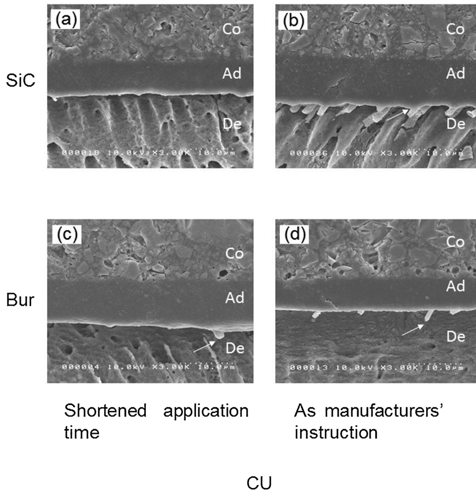
Fig. 3. SEM images of the interfacial structure of CU ( \times 3000 ) according to surface preparation and application time. (a) With shortened application time on SiC-ground dentine, no resin tags were observed. (b) Short resin tags (arrow) were observed when CU was applied according to manufacturers' instruction time on SiC-ground surface. (c, d) Few short resin tags (arrow) were formed in bur-cut dentine.
