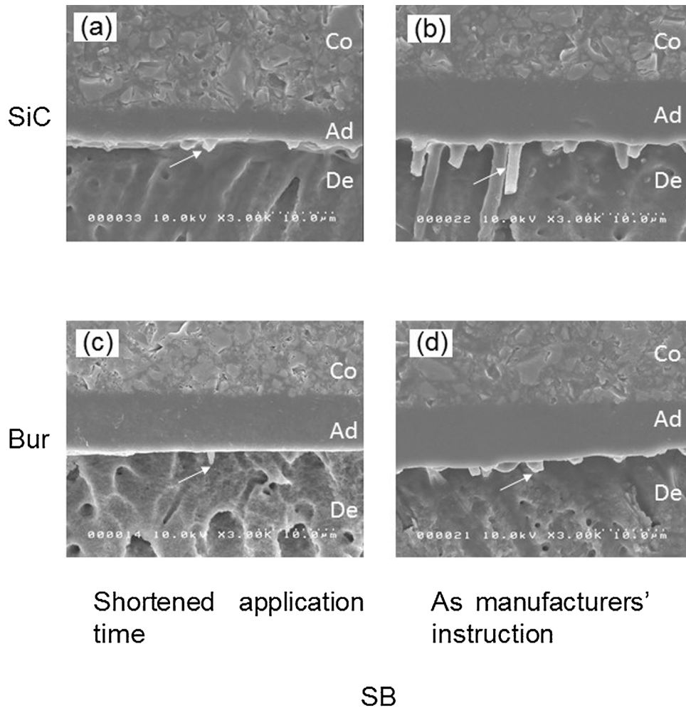
Fig. 5. SEM images of the interfacial structure of SB ( \times 3000 ) according to surface preparation and application time. (a) Poorly formed resin tags were observed with shortened application time group on SiC. (b) Longer and more tags (arrow) were observed when SB was applied according to manufacturers' instruction. (c) Only short resin tags were found on bur-cut dentine at shortened time. (d) More resin tags were detected when SB was applied according to manufacturers' instruction.
