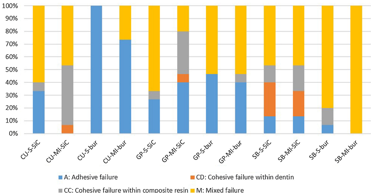
Fig. 1. Fracture modes of the three adhesives bonded to SiC prepared dentine and bur-cut dentine, with reduced application time and as manufacturers’ instruction.
