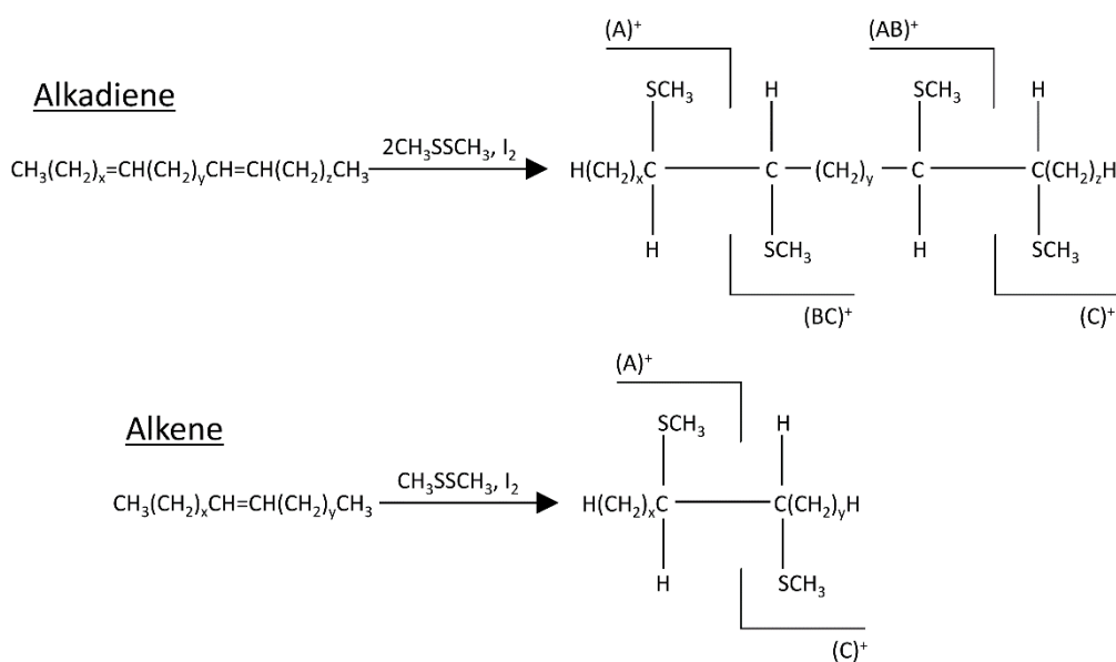
Fig.2.2 Fragmentation scheme for the formation of DMDS adducts of alkenes
