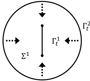
Figure 8: \Gamma_t^2 hits \Sigma^1
