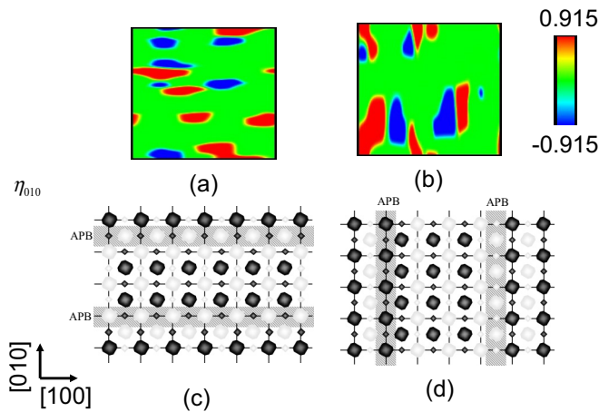
FIG. 6. The contour of the calculated long-range order parameters are displayed in (a) and (b). The atomic arrangements of L_{10} -ordered phase viewed from [001] are shown in (c) and (d), which correspond to (a) and (b), respectively. (a) and (c) [(b) and (d)] are \eta_{010} ( \eta_{100} ) variant.
