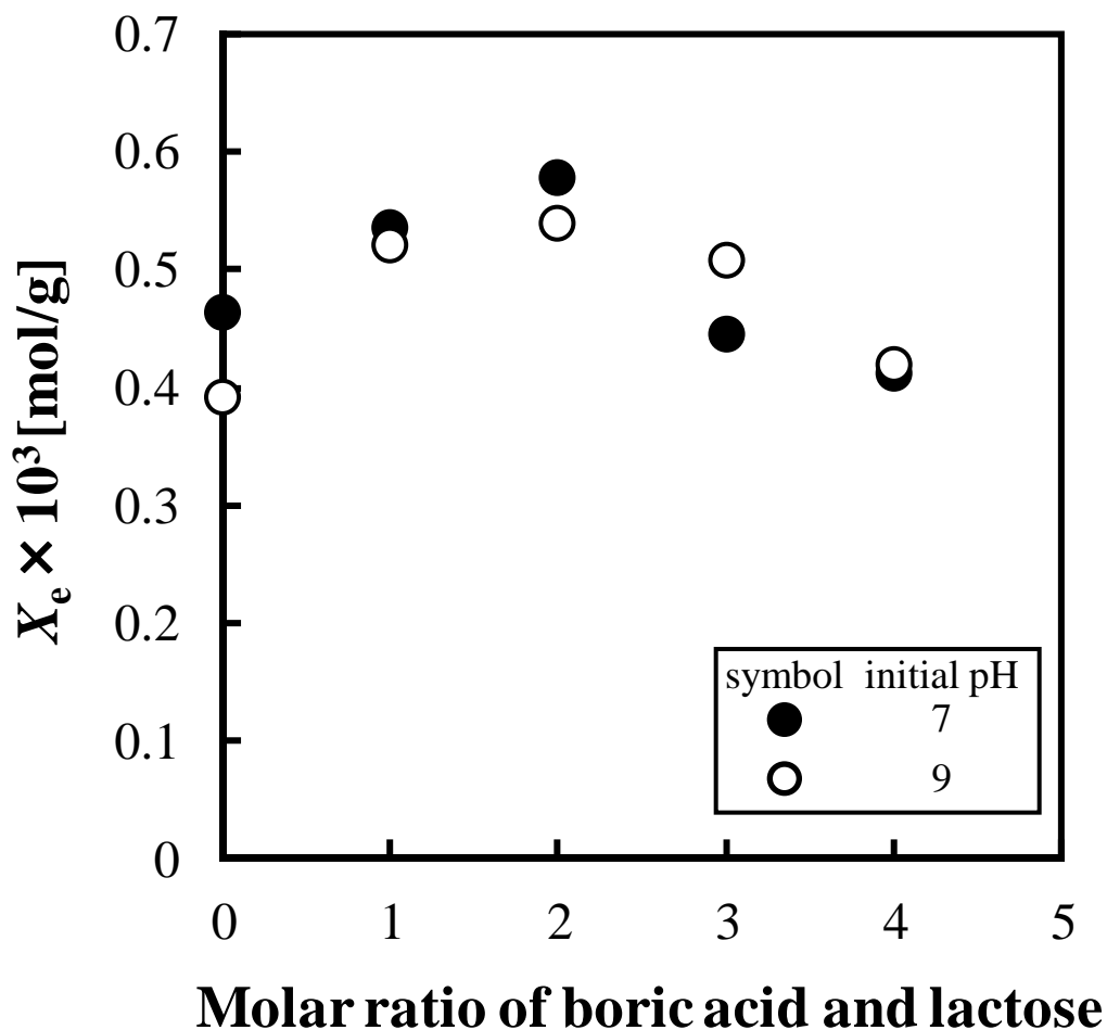
Fig. 4. Influence of the molar ratio of boric acid and lactose on the equilibrium adsorption density, X_e , onto anion exchange resin, IRA402, for initial pH 7 (●) and pH 9 (○) , respectively. Experimental conditions: lactose 0.01 M; IRA402 0.5 dry-g; solution volume 40 mL.
