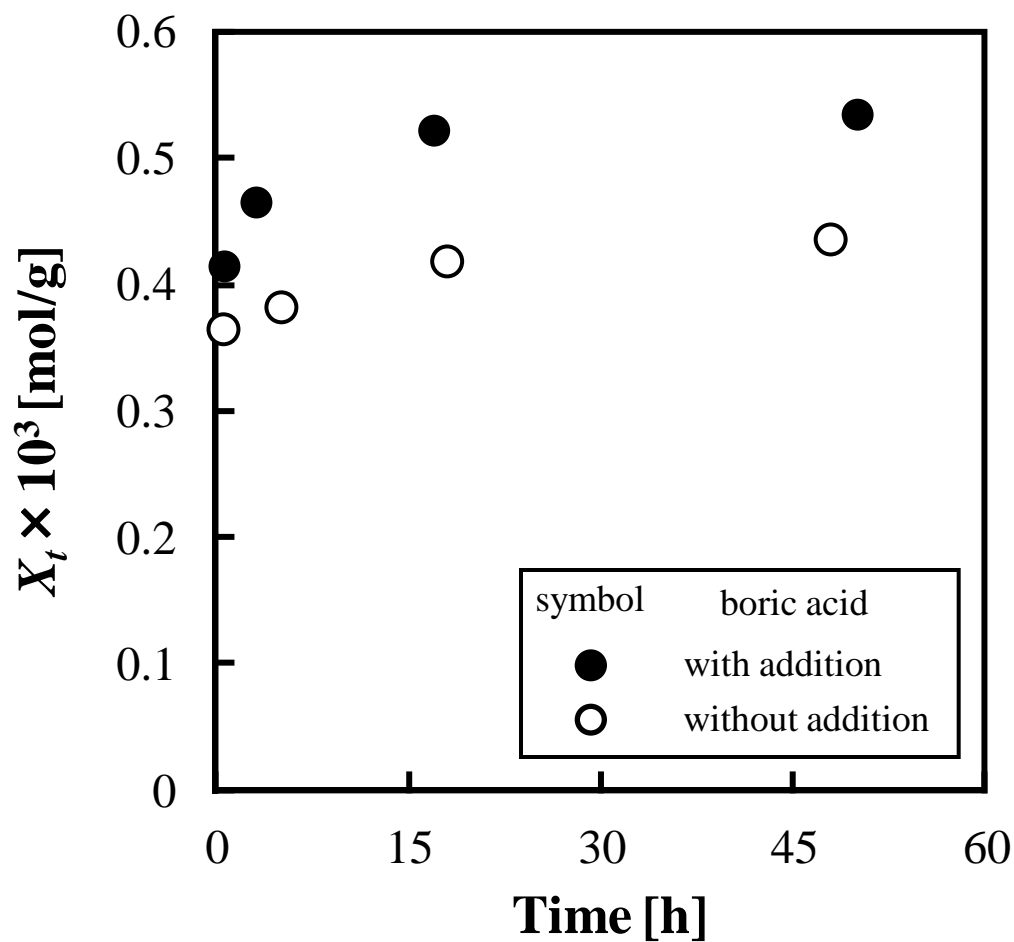
Fig. 2. Influence of boric acid on lactose adsorption onto IRA402 anion exchange resin. Experimental conditions: lactose 0.01 M; boric acid 0.01 M; solution volume 40 mL; IRA402 0.5 dry-g; initial pH 7.
