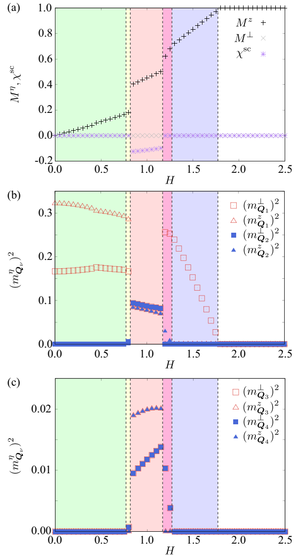
FIG. 3. H dependence of (a) the magnetization M^\eta and the scalar chirality \chi^{\text{sc}} , (b) \mathbf{Q}_1 and \mathbf{Q}_2 components of squared magnetic moments (m_{\mathbf{Q}_{1,2}}^\eta)^2 , and (c) \mathbf{Q}_3 and \mathbf{Q}_4 components of squared magnetic moments (m_{\mathbf{Q}_{3,4}}^\eta)^2 for \eta = \perp, z at I^A = 0.2 . The vertical dashed lines represent the phase boundaries between different spin states.
