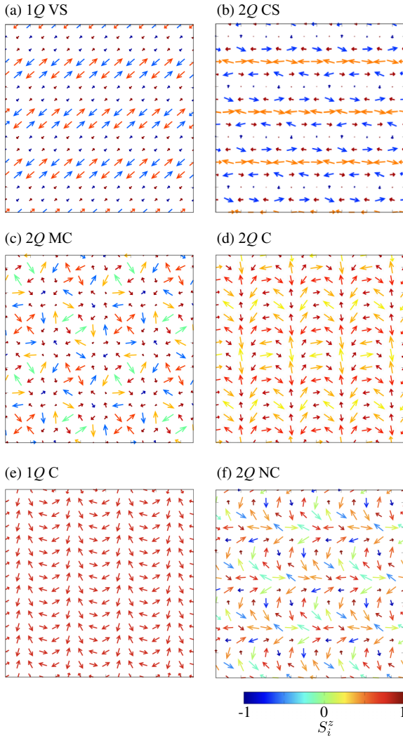
FIG. 4. Real-space spin configurations in (a) the 1 Q VS state at I^A = 0.2 and H = 0 , (b) the 2 Q CS state at I^A = 0.2 and H = 0.8 , (c) the 2 Q MC state at I^A = 0.2 and H = 1 , (d) the 2 Q C state at I^A = 0.2 and H = 1.2 , (e) the 1 Q C state at I^A = 0.2 and H = 1.4 , and (f) the 2 Q NC state at I^A = 0.1 and H = 0.7 . The arrows represent the direction of the in-plane spin and the color shows its z component.
