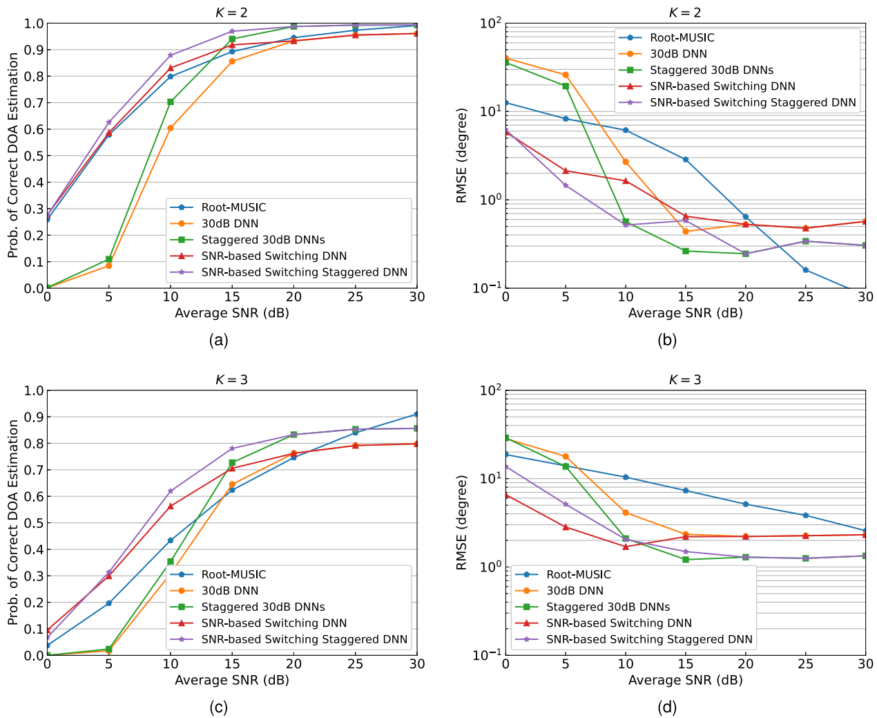
Fig. 10 Metrics comparison from same test dataset between Root-MUSIC and the two previous and two newly proposed DOA estimation methods. “30 dB DNN” corresponds to a DNN trained with a dataset generated from 30 dB data; “30 dB Staggered DNN” corresponds to DNN-A and DNN-B trained with a dataset generated from 30 dB data; “SNR-based Switching DNN” corresponds to the method of selecting the appropriate DNN based on SNR estimation; “SNR-based Switching Staggered DNN” is the method combining SNR-based Switching and Staggered DNNs. (a) Probability of correct DOA estimation when K = 2 . (b) RMSE when K = 2 . (c) Probability of correct DOA estimation when K = 3 . (d) RMSE when K = 3 .
