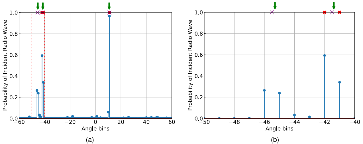
Fig. 5 (a) DNN output angle spectrum for a DNN trained offline at 30 dB and tested at 30 dB. Green arrows represent true DOAs, red thick crosses represent estimated DOAs by “Largest Search”, and purple thin crosses represent estimated DOAs by “Neighbors Average”. (b) Zoomed-in plot of (a) within the range [-50^\circ, -40^\circ] , highlighted by the red dotted rectangle.
