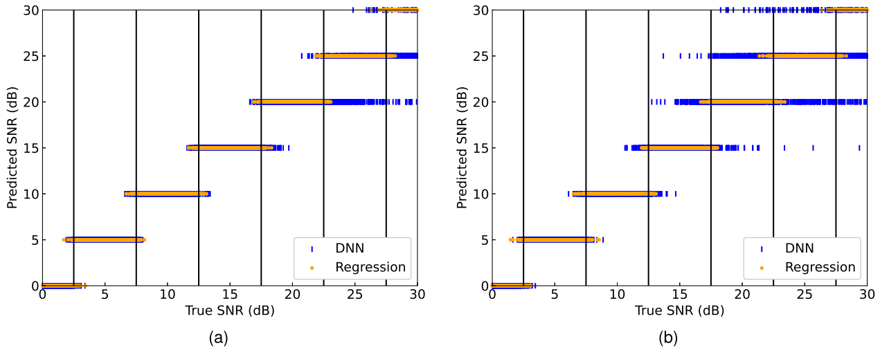
Fig. 8 SNR estimation performance comparison between DNN and linear regression obtained from 5,000 samples. The abscissa label “True SNR” corresponds to the SNR manually set during simulation. (a) K = 2 . (b) K = 3 .
