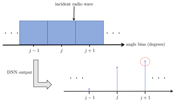
Fig. 3 Consequence of radio waves incident on the angle bin border. The j + 1 bin is mistakenly detected as the true DOA.
