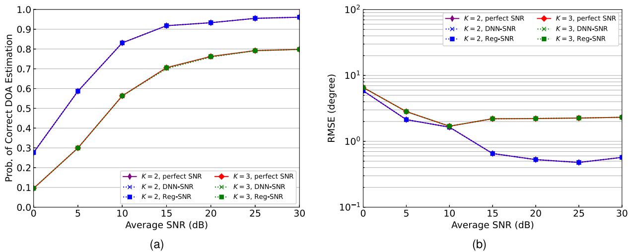
Fig. 9 DOA detection accuracy comparison with the “SNR-based Switching DNN” method when the SNR estimator module is perfect, DNN-based, and regression-based, for the cases K = 2 and 3. (a) Probability of correct DOA estimation. (b) RMSE.
