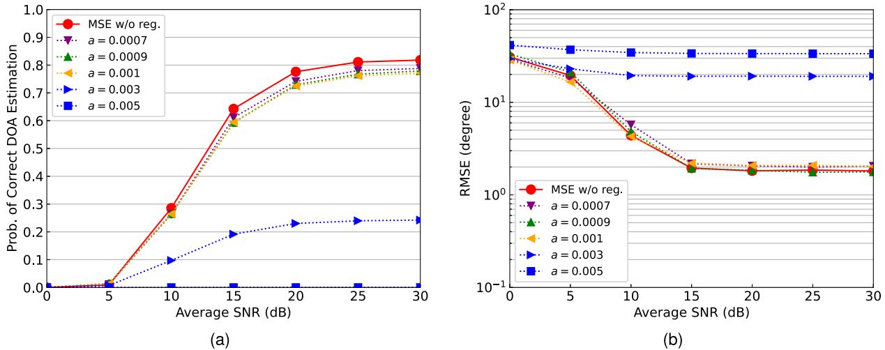
Fig. 12 Performance analysis of the DOA estimator when the MSE loss is regularized by an l_p -norm term, for the case p = 0.95 , and varying scaling factor a . Comparison is also made with the case when no regularization term is added. (a) Probability of correct DOA estimation. (b) RMSE.
