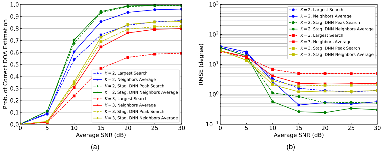
Fig. 7 Estimation accuracy improvement by the proposed technique named “Neighbors Average”. (a) Probability of correct DOA estimation. (b) RMSE.
