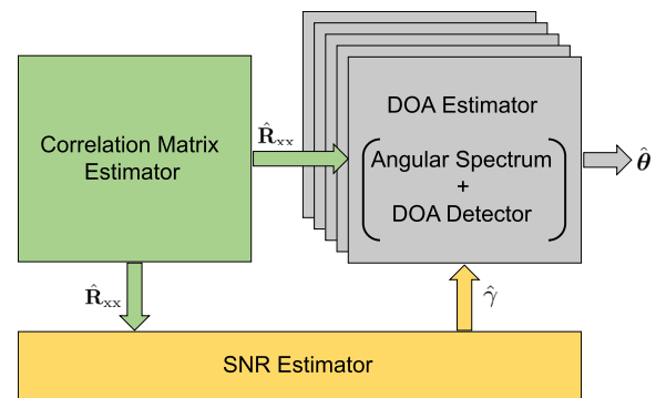
Fig. 6 Schematics of the proposed SNR-based Switching DNN.
