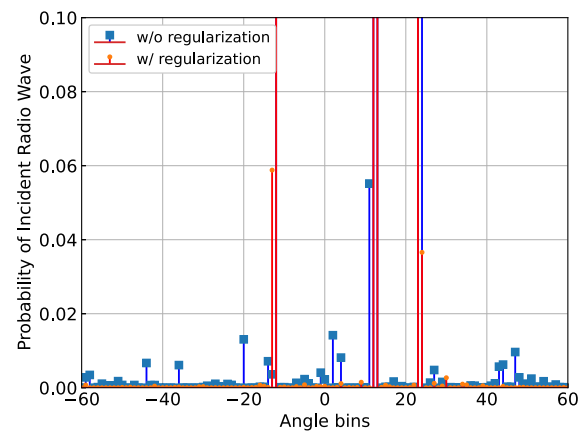
Fig. 13 Comparison of the DNN output angular spectrum obtained by a DNN trained with and without the regularization l_p -norm, when p = 0.95 and a = 0.0009 . For better visualization, this graph is plotted until the probability of success of 0.10. Successful DOA detection is achieved in both cases.
