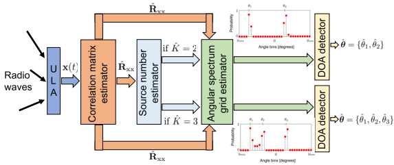
Fig. 1 Proposed system schematics where \hat{K} and \hat{\theta} denote estimated values of the number of sources and DOAs, respectively.
