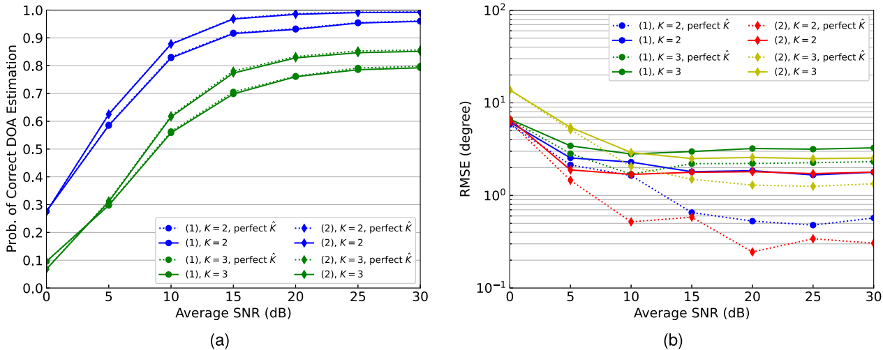
Fig. 11 Proposed system performance comparison when source number estimation is perfect ( \hat{K} ) and not perfect, and when SNR-based (1) Switching DNN or (2) Switching Staggered DNNs are used as spectrum estimation techniques. SNR estimation is done with the regression-based method. (a) Probability of correct DOA estimation. (b) RMSE.
