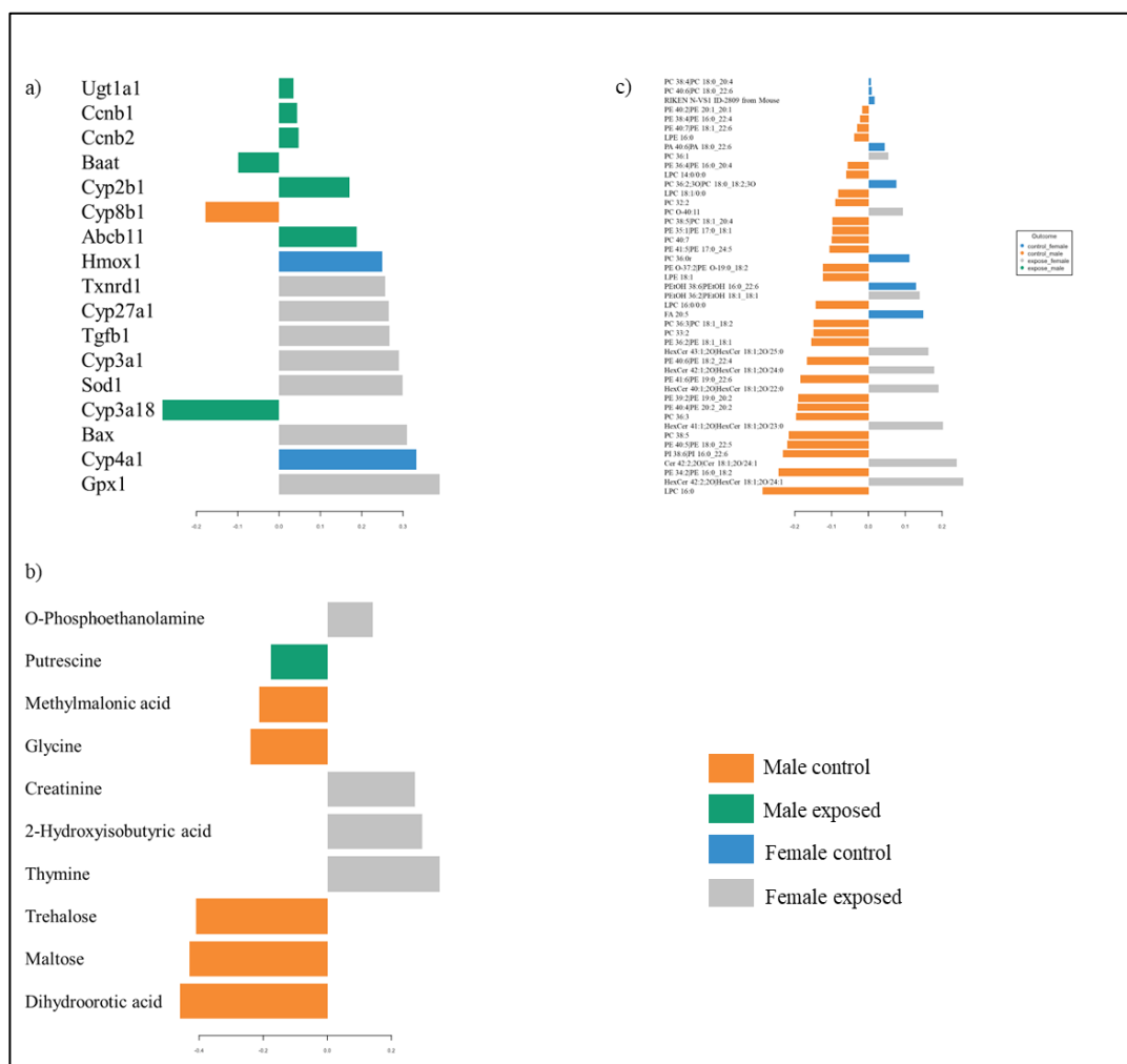
Figure 3.8. Contribution scores for component 1. Contribution scores of the selected variables for component 1 are shown using a bar plot. The bar length reflects the importance of each variable in this model, and its direction indicates a positive or negative coefficient for each variable. The bar color indicates the rat groups which has the highest mean of each variable.
